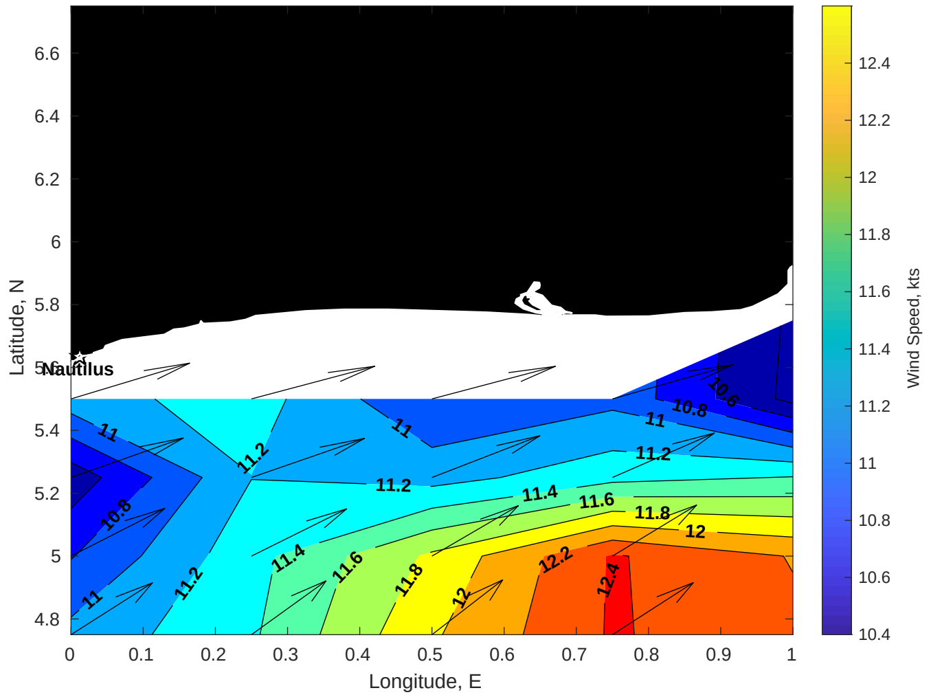
Winds (kts) for Nautilus at 01-Aug-2025 09:00:00
