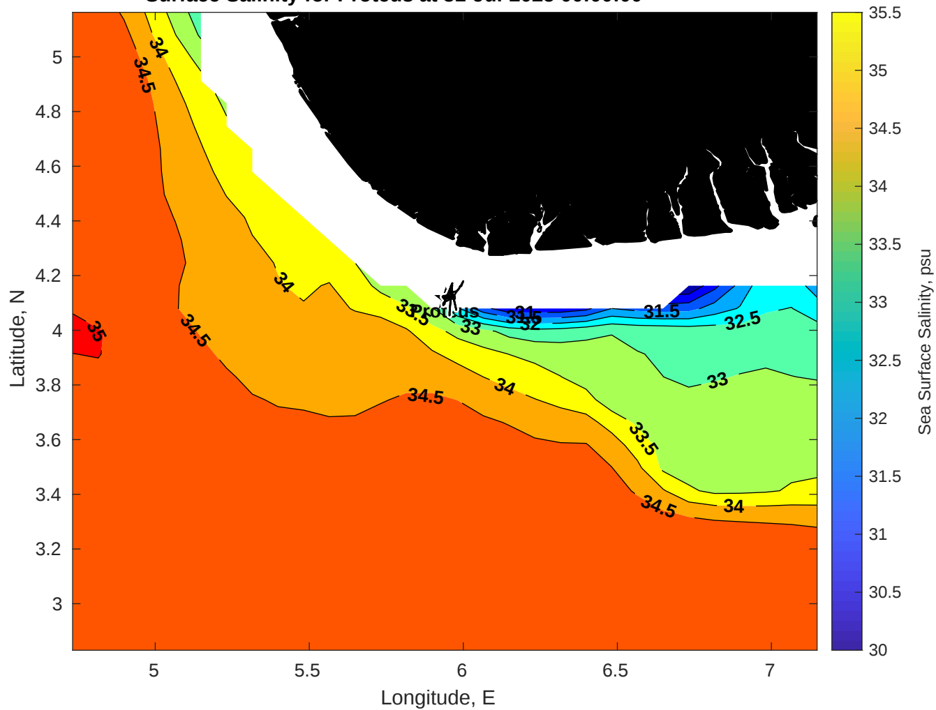
Surface Salinity for Proteus at 31-Jul-2025 00:00:00
