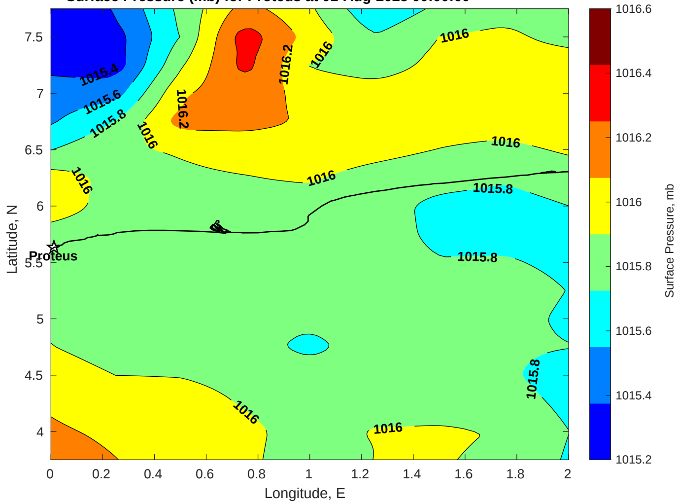
Surface Pressure (mb) for Proteus at 01-Aug-2025 00:00:00
