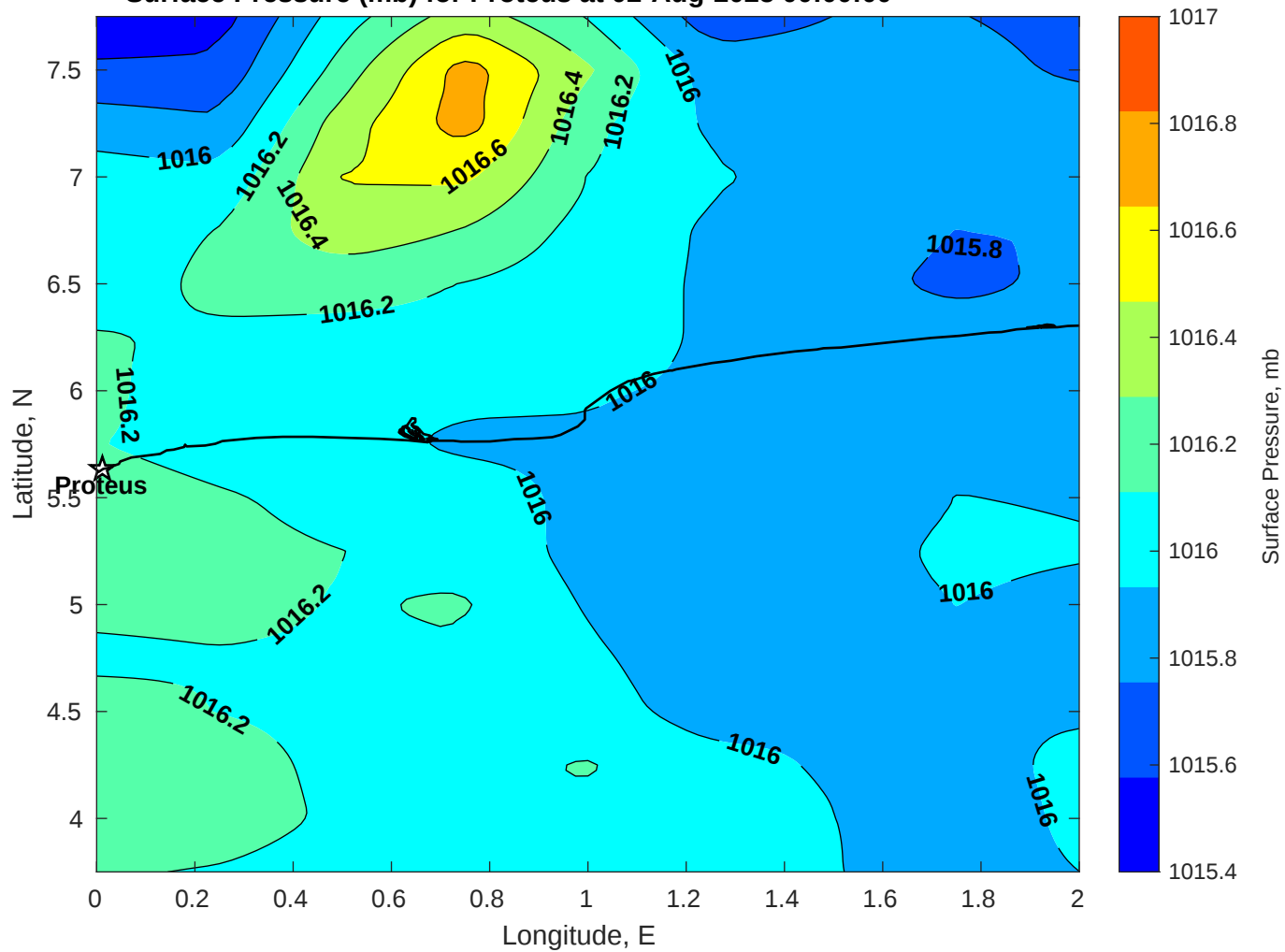
Surface Pressure (mb) for Proteus at 02-Aug-2025 00:00:00
