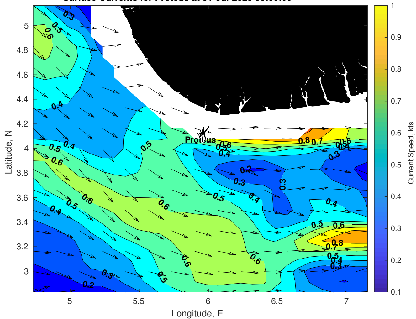
Surface Currents for Proteus at 31-Jul-2025 00:00:00
