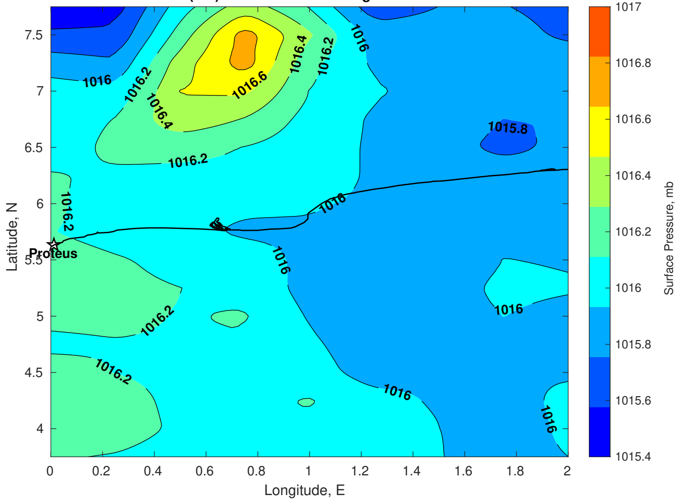
Surface Pressure (mb) for Proteus at 02-Aug-2025 00:00:00
