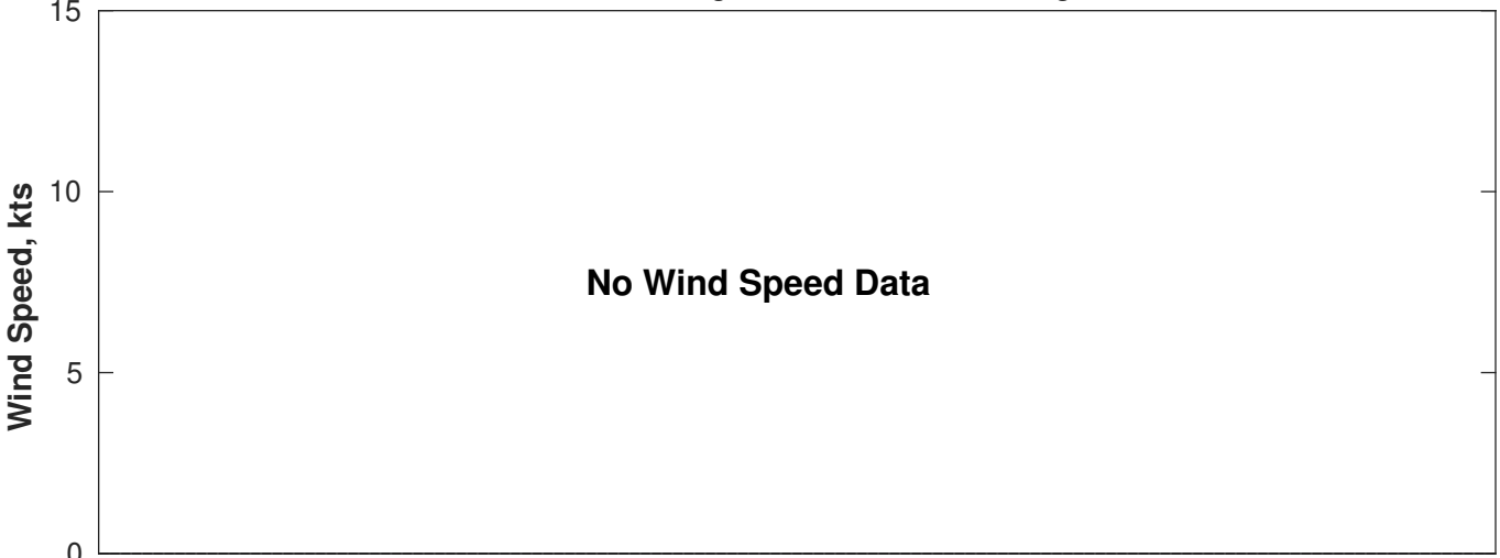
Wind & Wave Forecast for Proteus from 01-Aug-2025 01:00:00 to 17-Aug-2025 01:00:00
