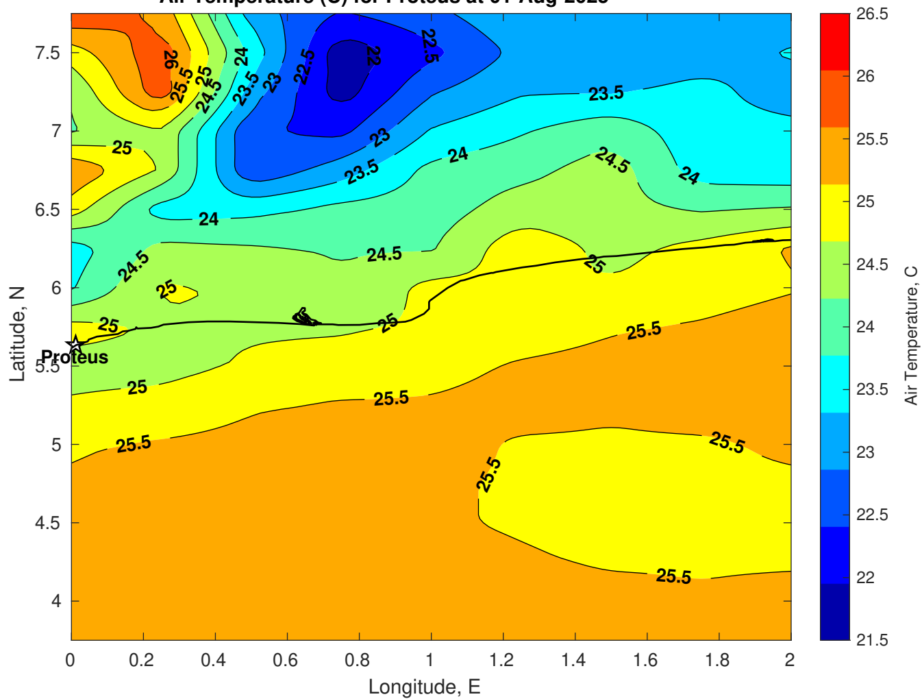
Air Temperature (C) for Proteus at 01-Aug-2025
