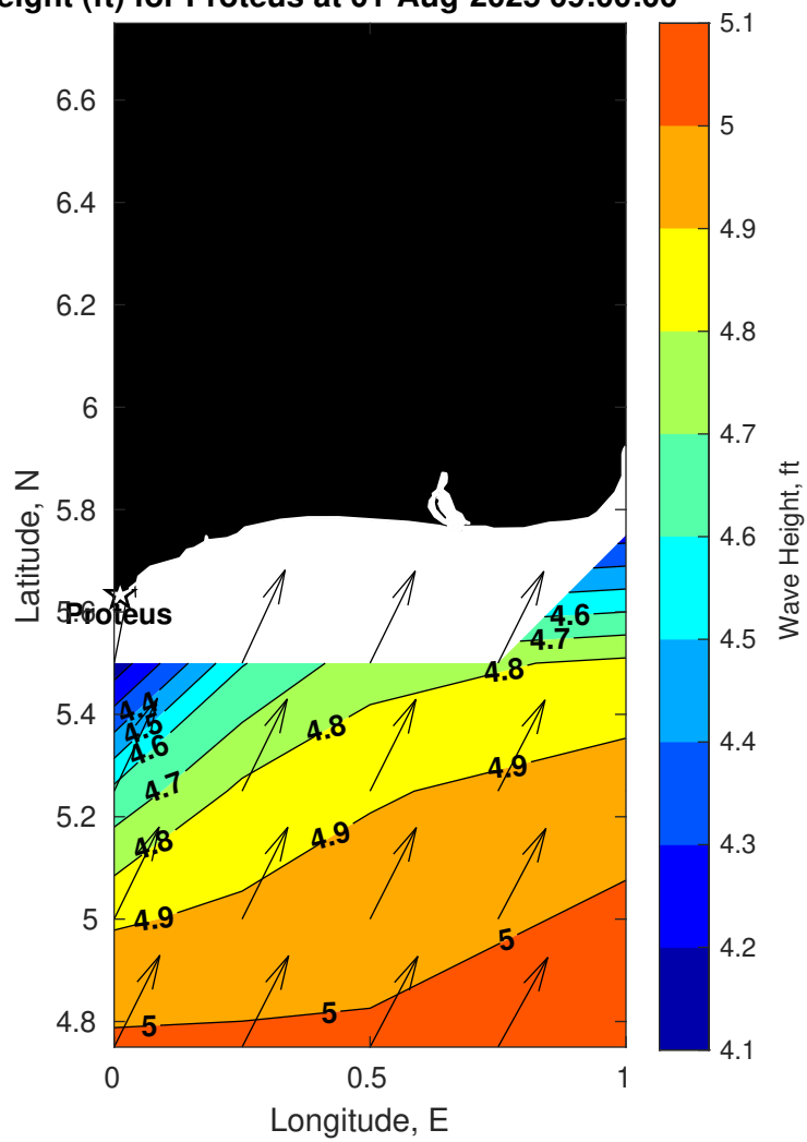
Wave Height (ft) for Proteus at 01-Aug-2025 09:00:00
