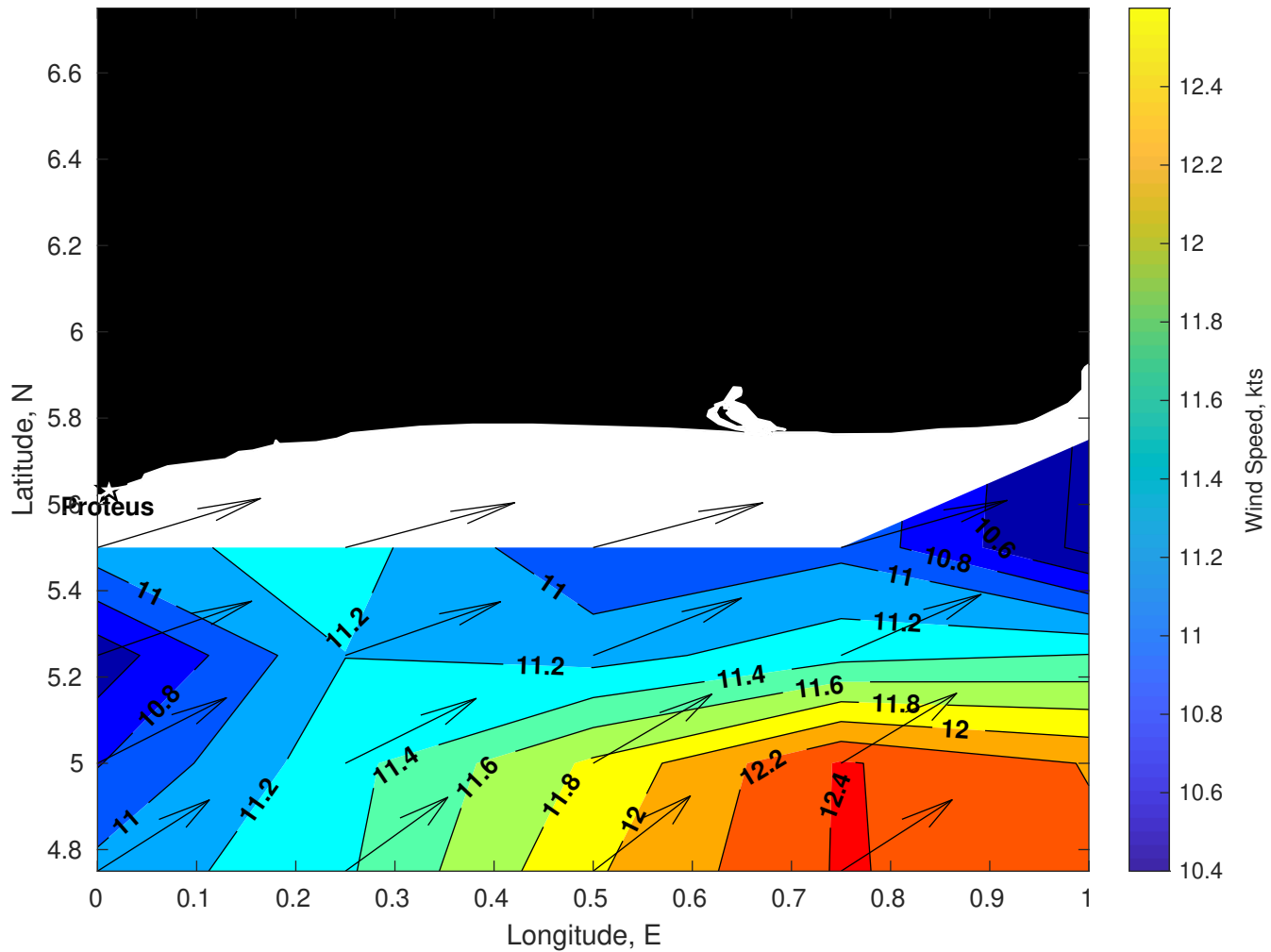
Winds (kts) for Proteus at 01-Aug-2025 09:00:00
