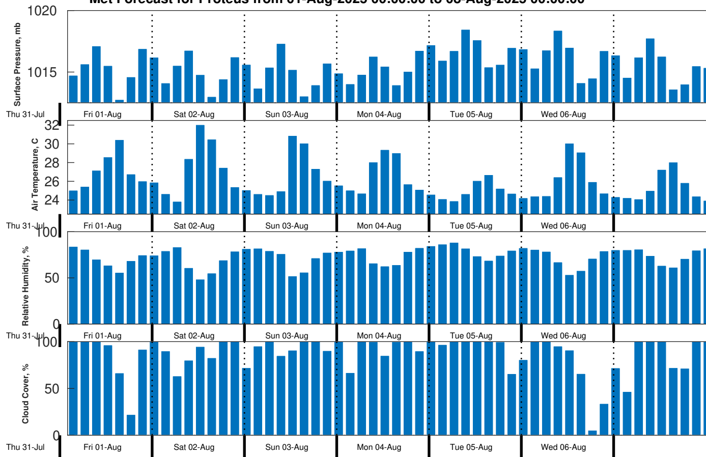
Met Forecast for Proteus from 01-Aug-2025 00:00:00 to 08-Aug-2025 00:00:00
