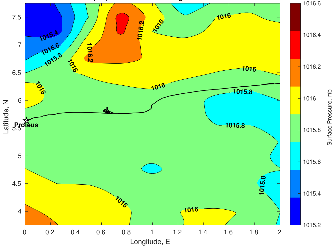
Surface Pressure (mb) for Proteus at 01-Aug-2025 00:00:00
