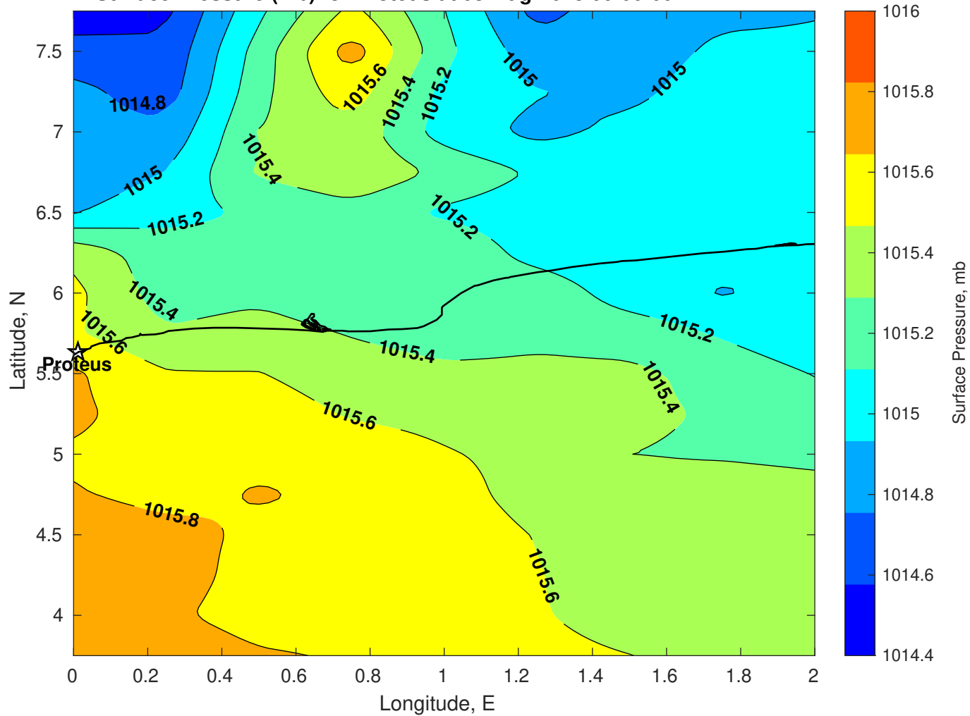
Surface Pressure (mb) for Proteus at 03-Aug-2025 00:00:00
