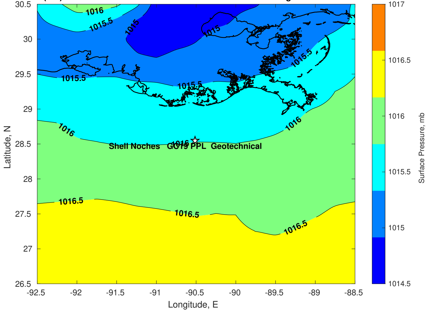
Surface Pressure (mb) for Shell Noches GC19 PPL Geotechnical at 01-Aug-2025 00:00:00
