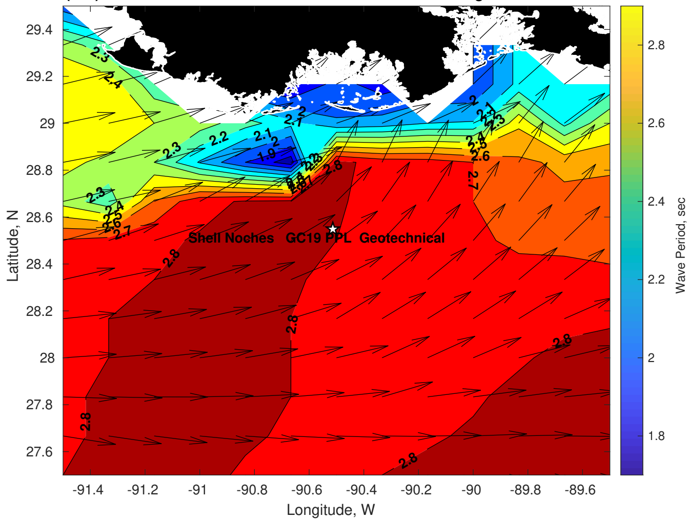
Wave Period (sec) for Shell Noches GC19 PPL Geotechnical at 01-Aug-2025 09:00:00
