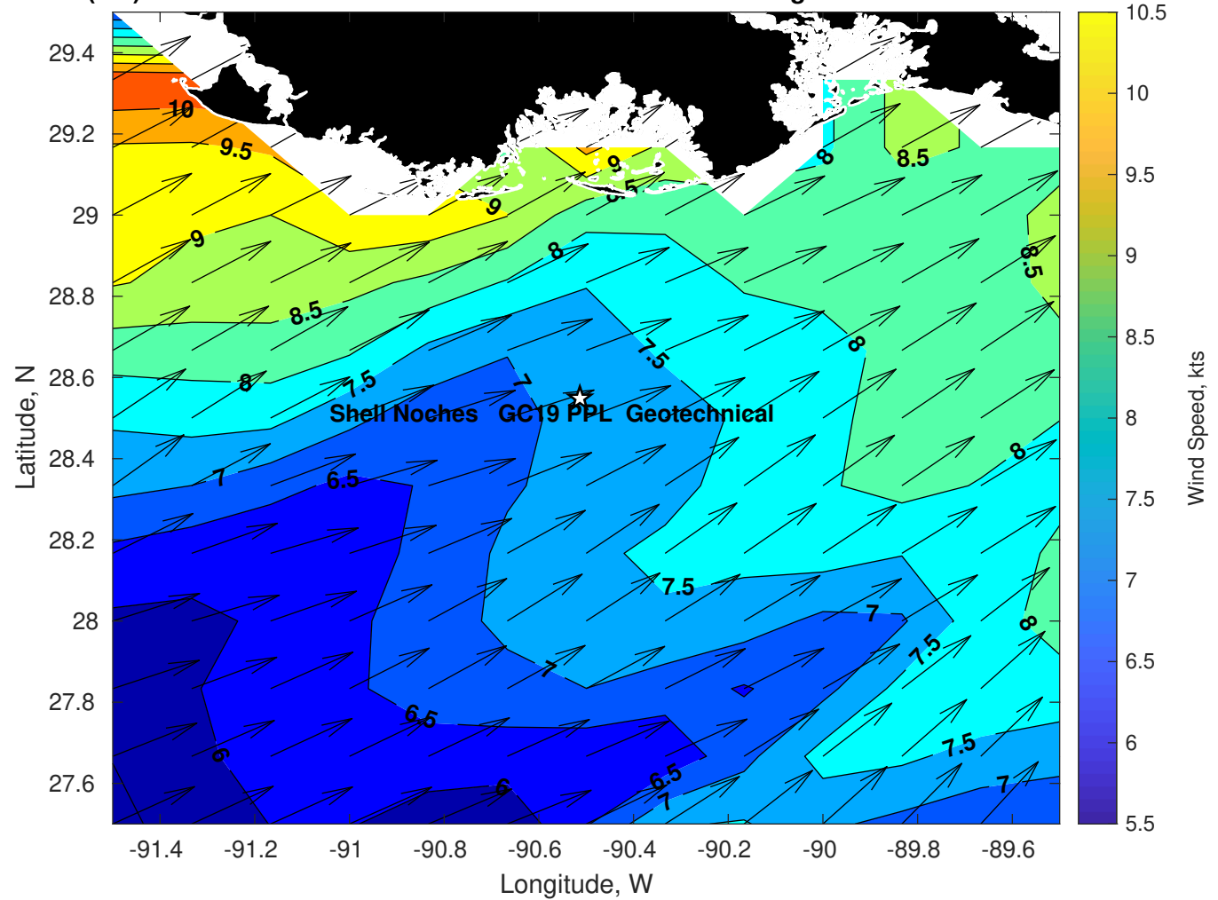
Winds (kts) for Shell Noches GC19 PPL Geotechnical at 01-Aug-2025 09:00:00
