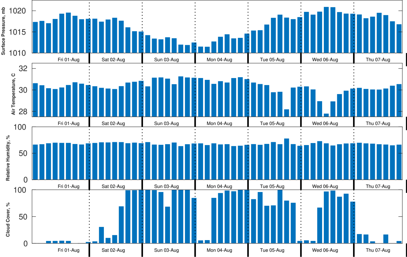
Met Forecast for Shell Noches GC19 PPL Geotechnical from 01-Aug-2025 00:00:00 to 08-Aug-2025 00:00:00
