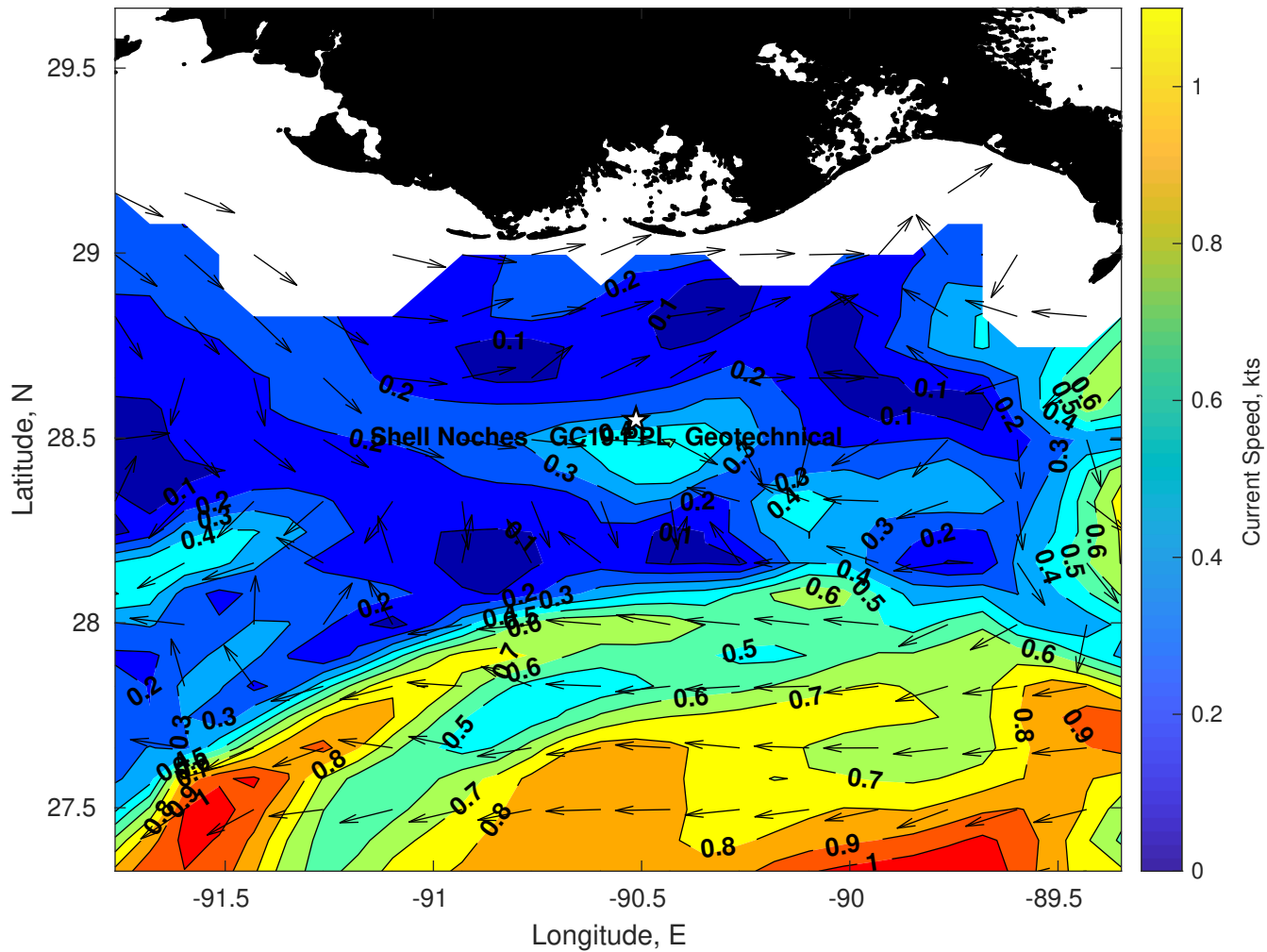
Surface Currents for Shell Noches GC19 PPL Geotechnical at 31-Jul-2025 00:00:00
