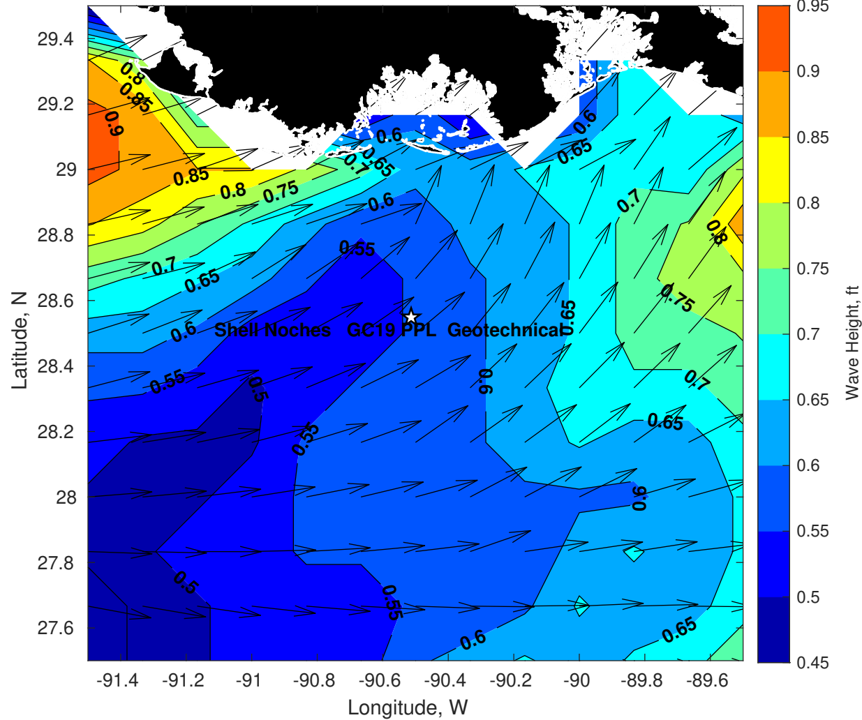
Wave Height (ft) for Shell Noches GC19 PPL Geotechnical at 01-Aug-2025 09:00:00
