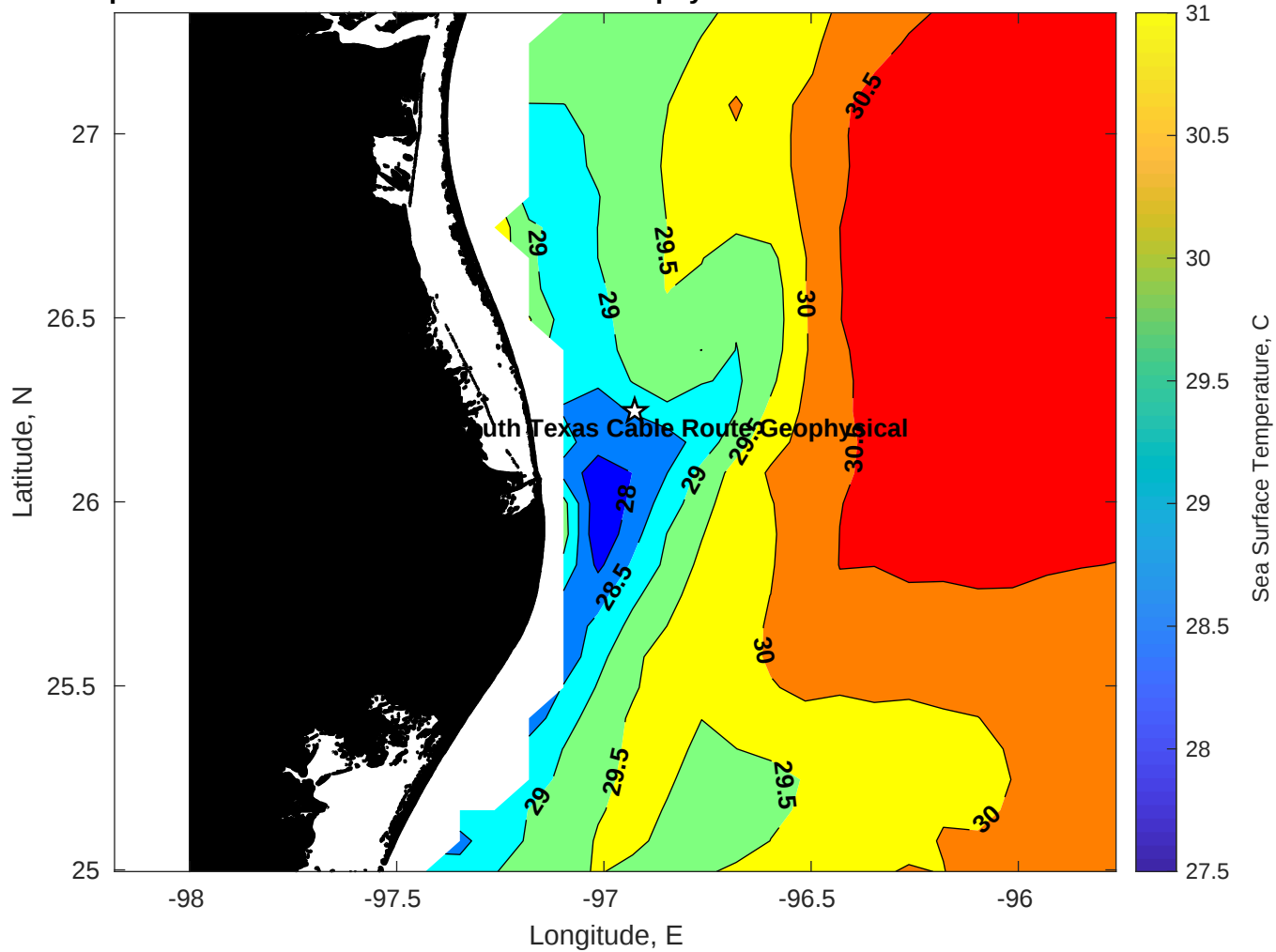
SST for Tampnet P2378 South Texas Cable Route Geophysical at 31-Jul-2025 00:00:00
