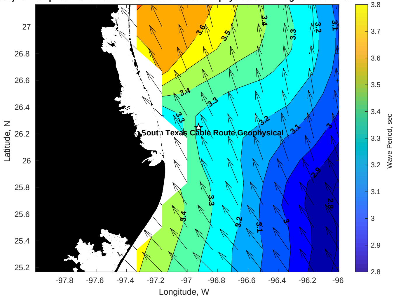
Period (sec) for Tampnet P2378 South Texas Cable Route Geophysical at 01-Aug-2025 09:00:00
