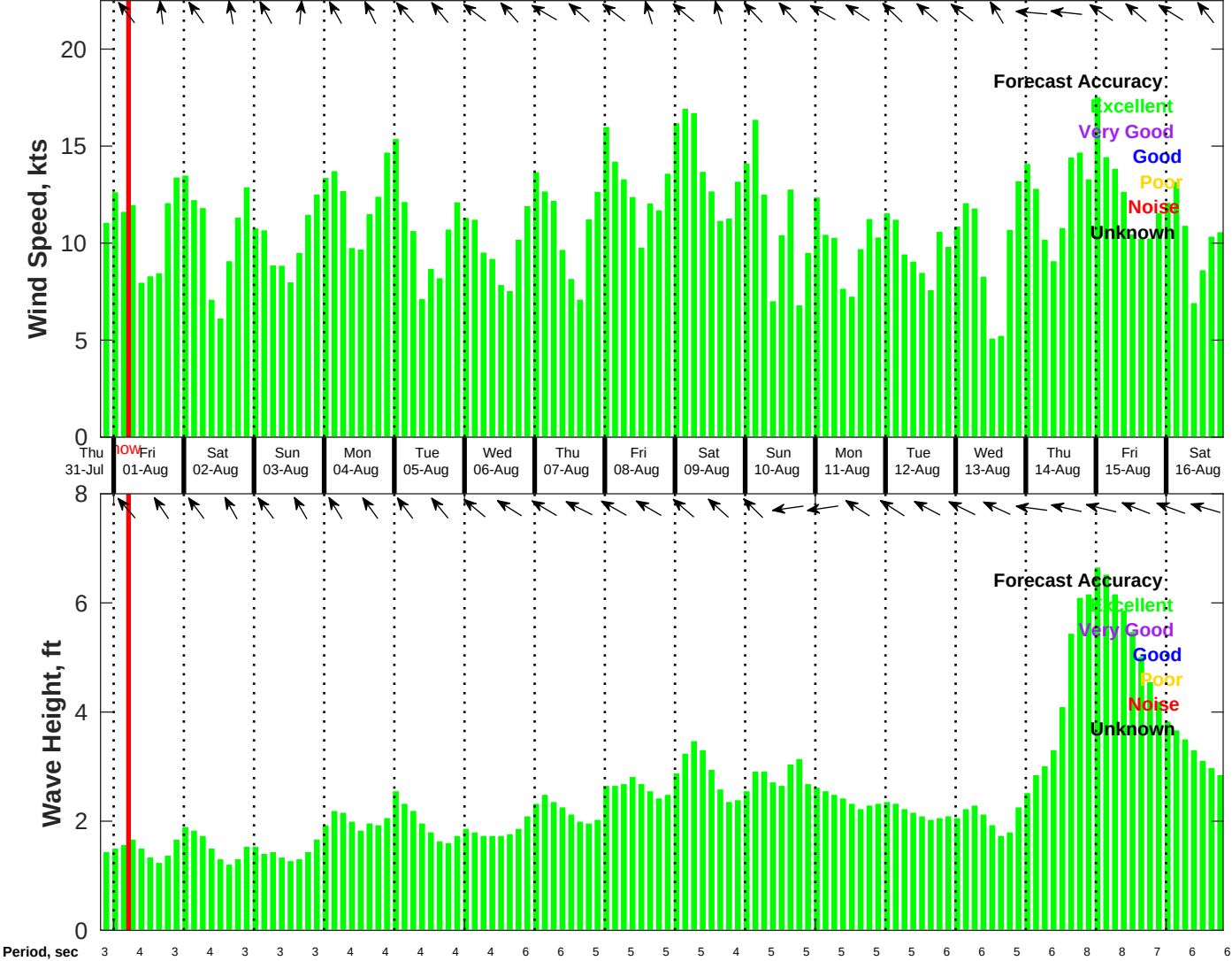
Wind & Wave Forecast for Tampnet P2378 South Texas Cable Route Geophysical from 31-Jul-2025 20:00:00 to 16-Aug-2025 20:00:00
