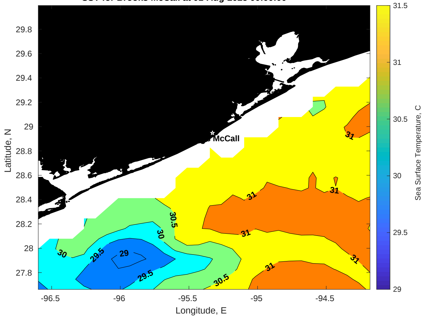
SST for Brooks McCall at 01-Aug-2025 00:00:00
