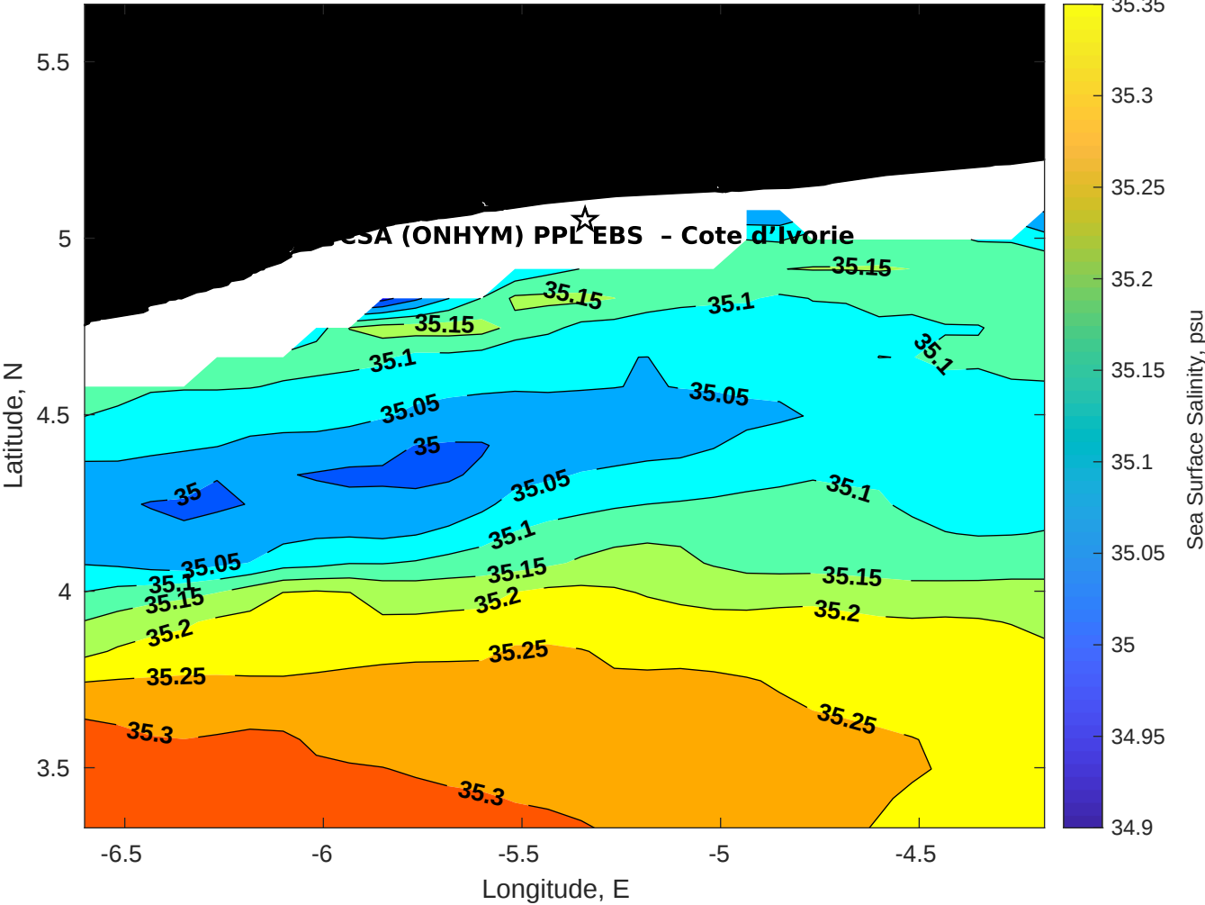
Surface Salinity for CSA (ONHYM) PPL EBS - Cote d'Ivoire at 01-Aug-2025 00:00:00
