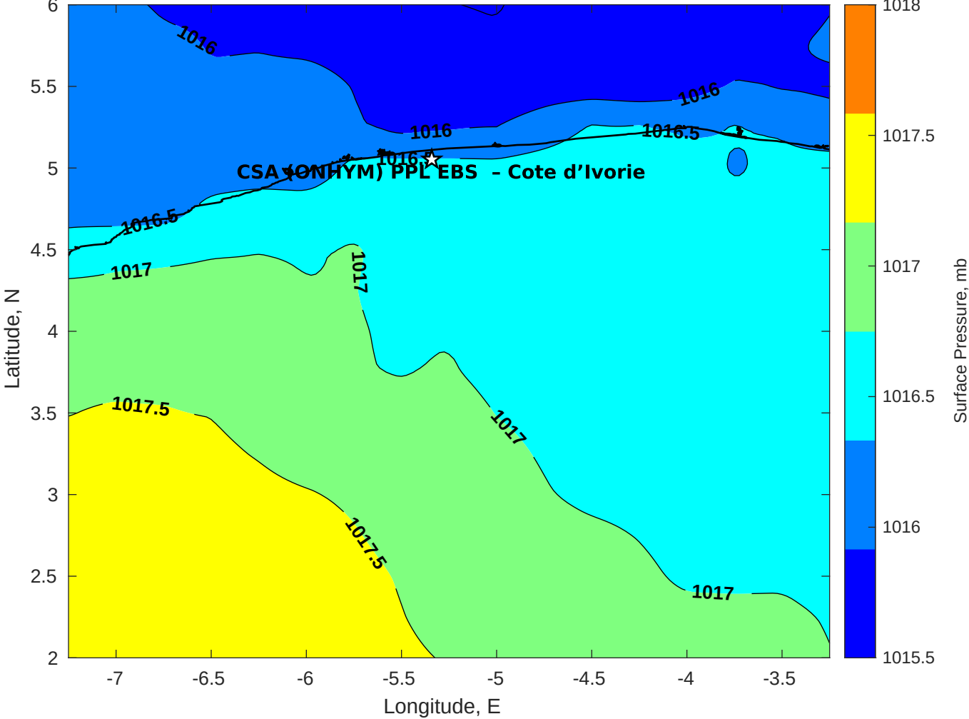
Surface Pressure (mb) for CSA (ONHYM) PPL EBS - Cote d'Ivoire at 03-Aug-2025 12:00:00
