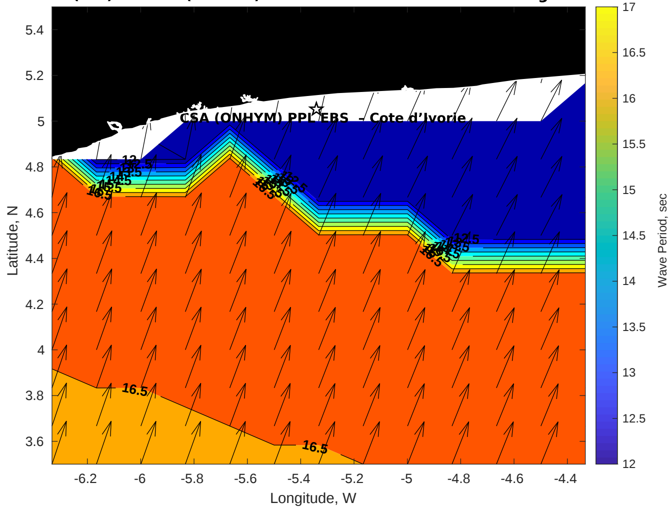
Wave Period (sec) for CSA (ONHYM) PPL EBS - Cote d'Ivoire at 01-Aug-2025 21:00:00
