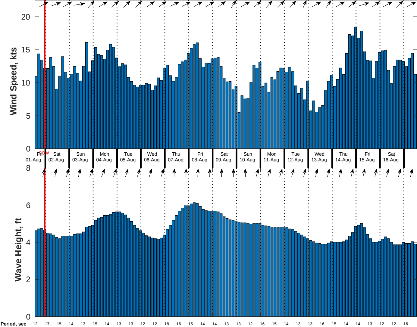
Wind & Wave Forecast for CSA (ONHYM) PPL EBS - Cote d'Ivoire from 01-Aug-2025 13:00:00 to 17-Aug-2025 13:00:00
