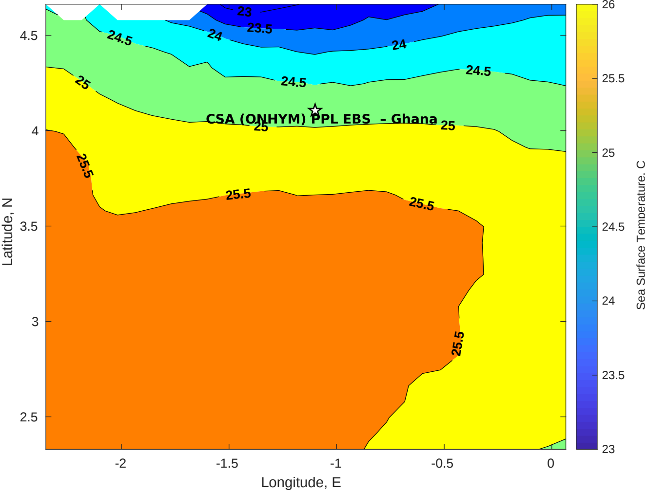
SST for CSA (ONHYM) PPL EBS - Ghana at 01-Aug-2025 00:00:00
