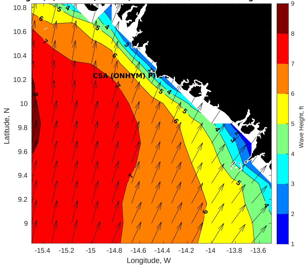
Wave Height (ft) for CSA (ONHYM) PPL EBS - Guinea at 01-Aug-2025 21:00:00
