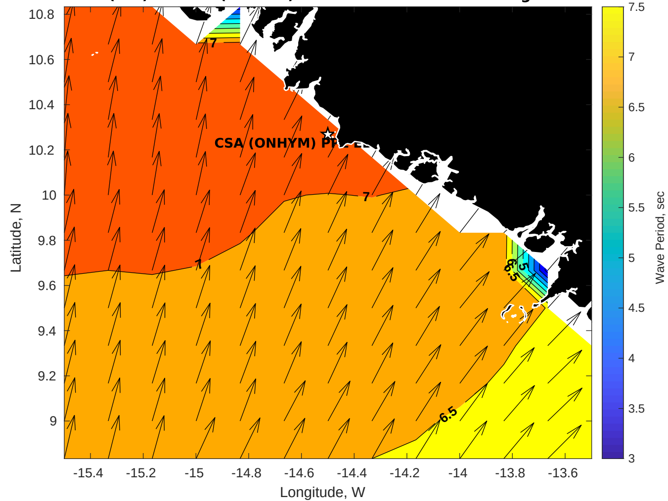
Wave Period (sec) for CSA (ONHYM) PPL EBS - Guinea at 01-Aug-2025 21:00:00
