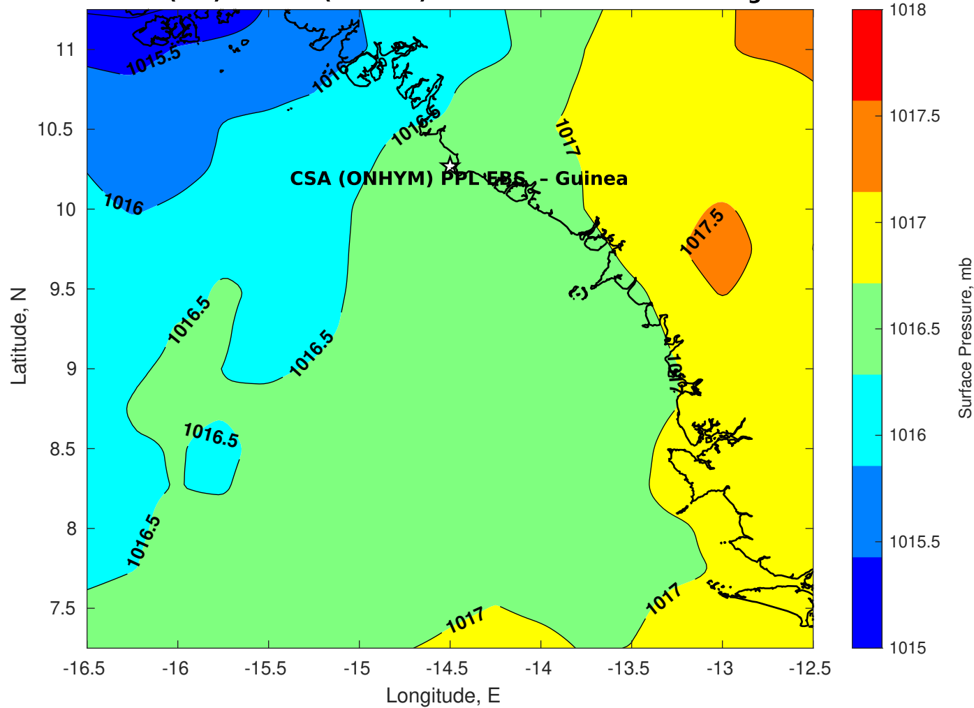
Surface Pressure (mb) for CSA (ONHYM) PPL EBS - Guinea at 02-Aug-2025 12:00:00
