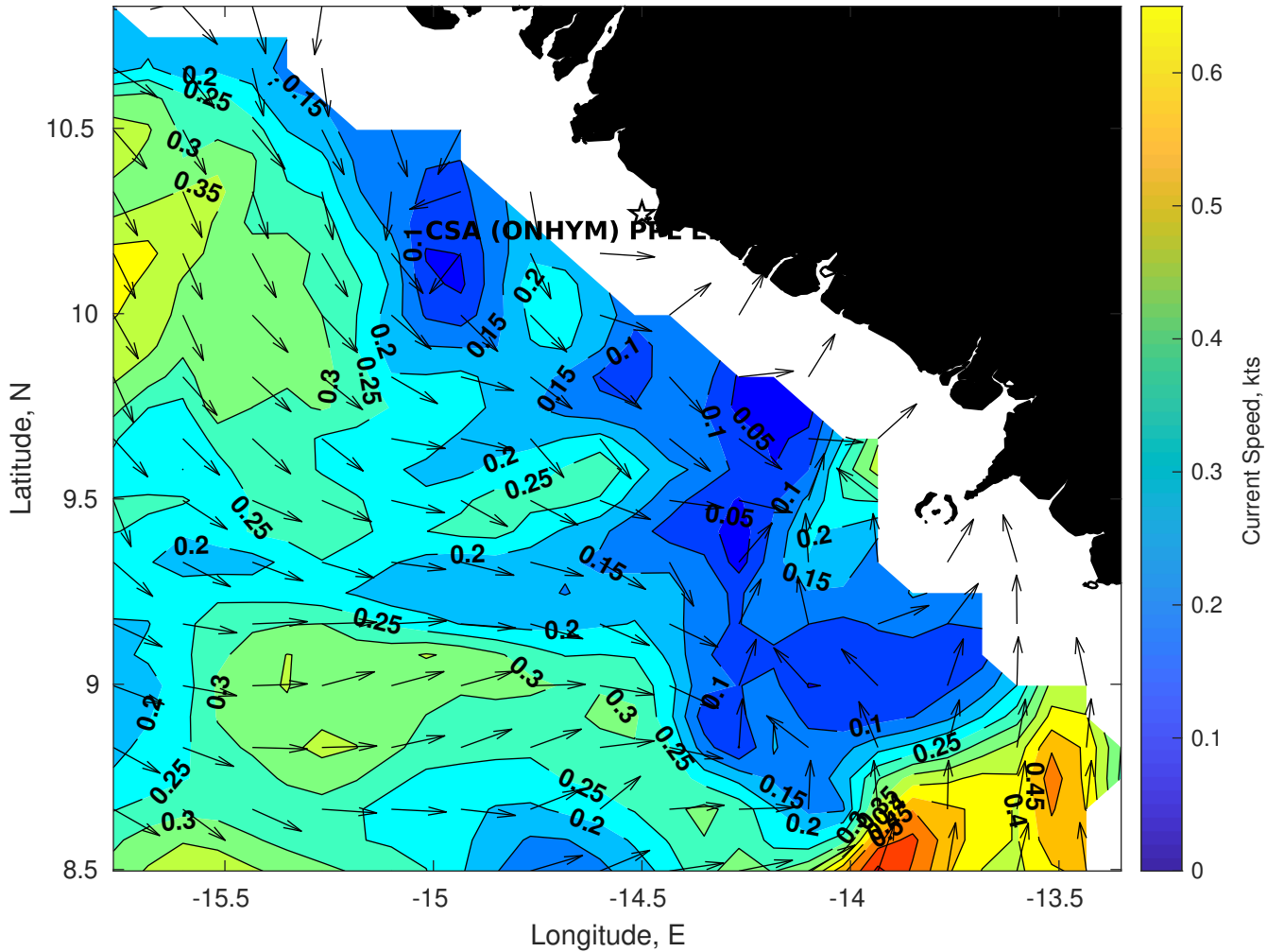
Surface Currents for CSA (ONHYM) PPL EBS - Guinea at 01-Aug-2025 00:00:00
