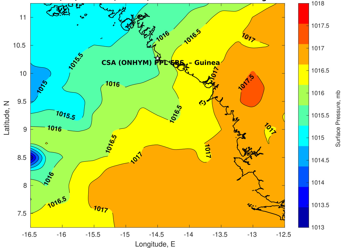
Surface Pressure (mb) for CSA (ONHYM) PPL EBS - Guinea at 01-Aug-2025 12:00:00
