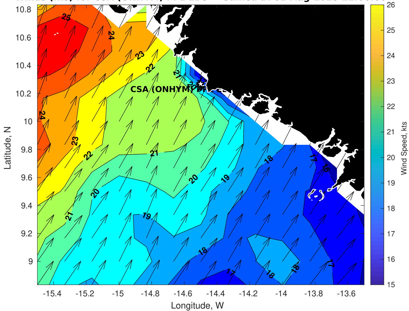
Winds (kts) for CSA (ONHYM) PPL EBS - Guinea at 01-Aug-2025 21:00:00
