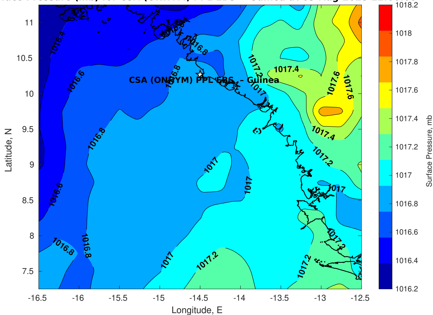
Surface Pressure (mb) for CSA (ONHYM) PPL EBS - Guinea at 03-Aug-2025 12:00:00
