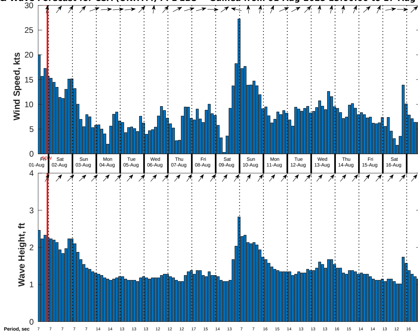
Wind & Wave Forecast for CSA (ONHYM) PPL EBS - Guinea from 01-Aug-2025 13:00:00 to 17-Aug-2025 13:00:00
