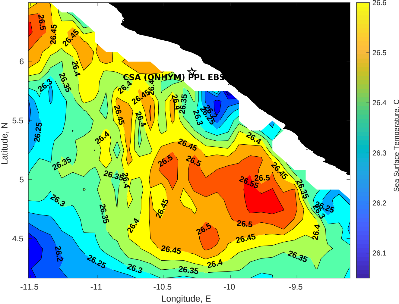
SST for CSA (ONHYM) PPL EBS - Liberia at 01-Aug-2025 00:00:00
