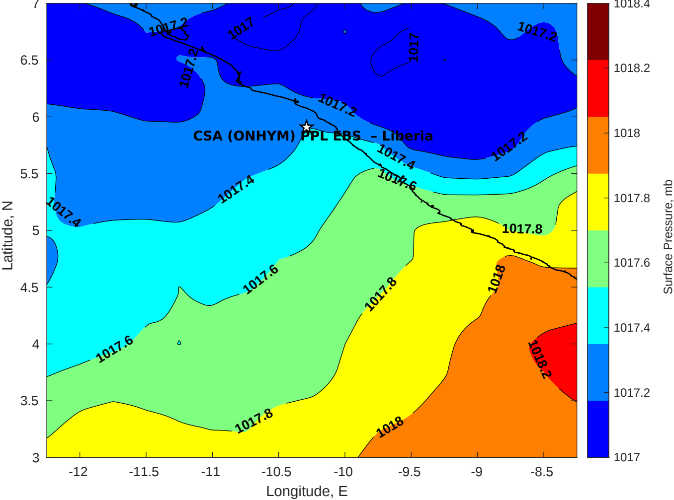
Surface Pressure (mb) for CSA (ONHYM) PPL EBS - Liberia at 02-Aug-2025 12:00:00
