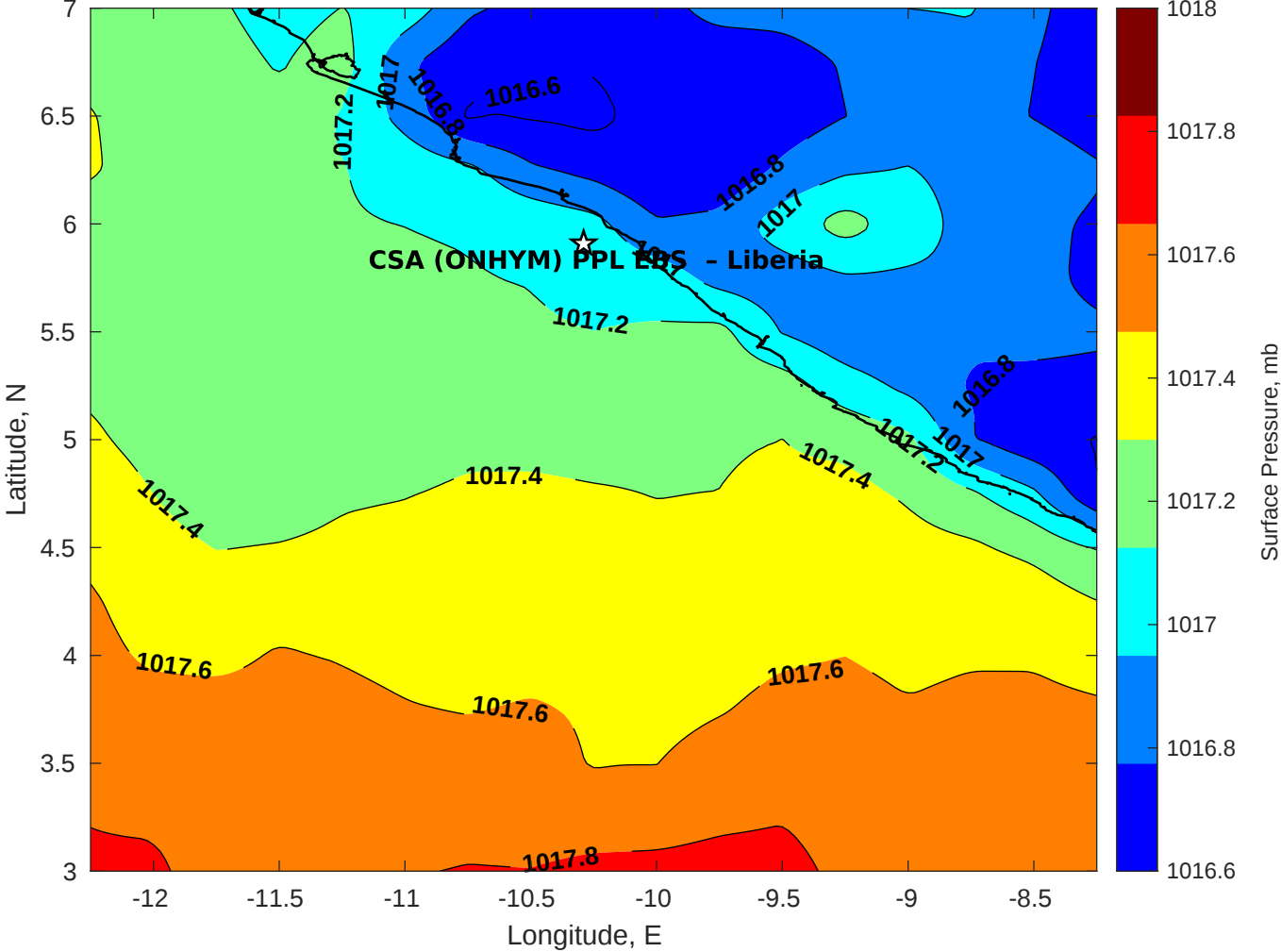
Surface Pressure (mb) for CSA (ONHYM) PPL EBS - Liberia at 03-Aug-2025 12:00:00
