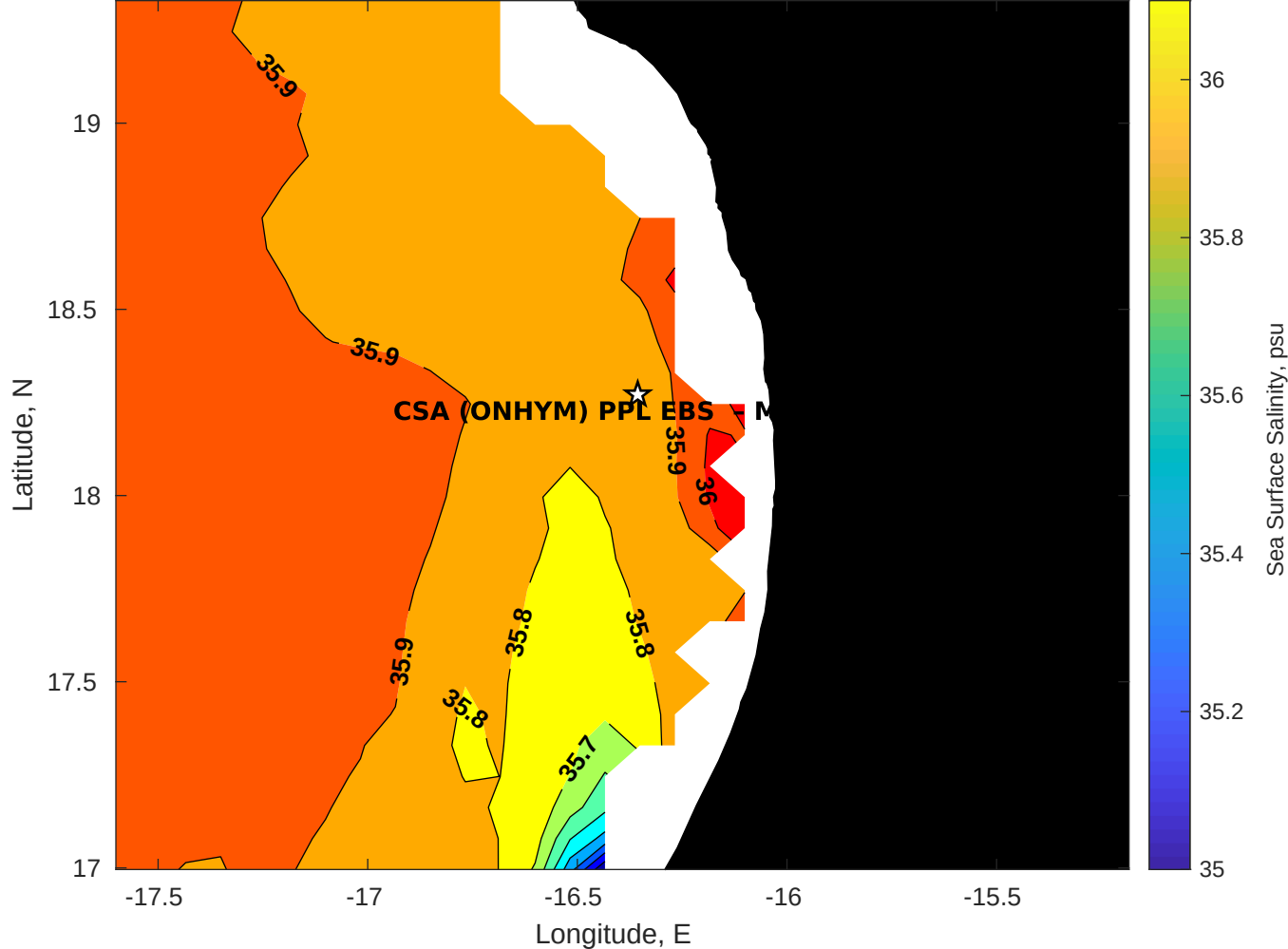
Surface Salinity for CSA (ONHYM) PPL EBS - Mauritania at 01-Aug-2025 00:00:00
