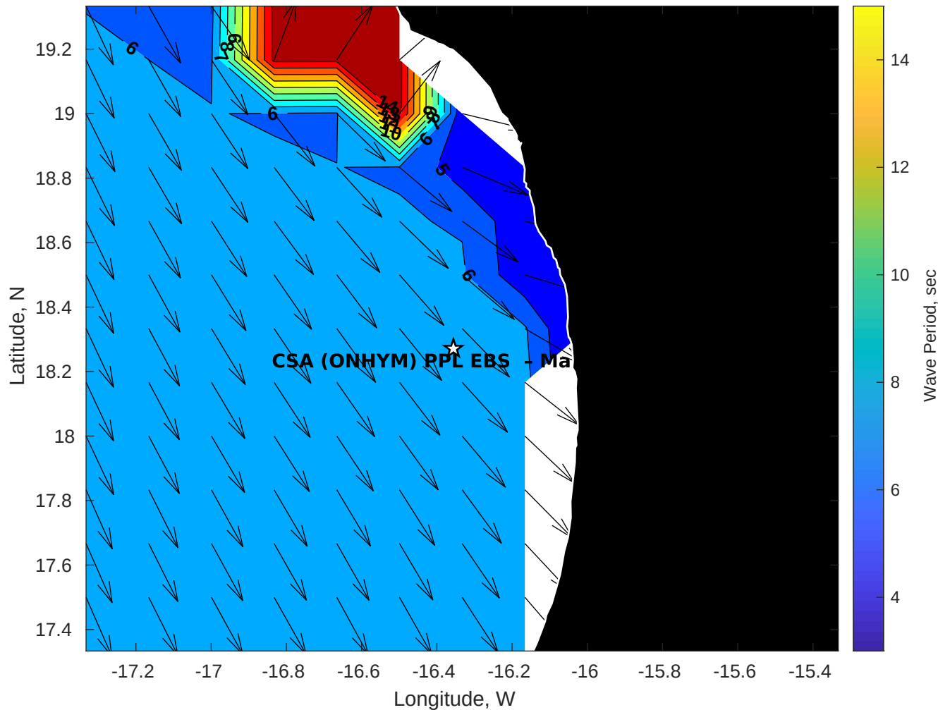
Wave Period (sec) for CSA (ONHYM) PPL EBS - Mauritania at 01-Aug-2025 21:00:00
