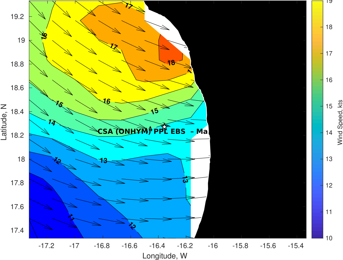
Winds (kts) for CSA (ONHYM) PPL EBS - Mauritania at 01-Aug-2025 21:00:00
