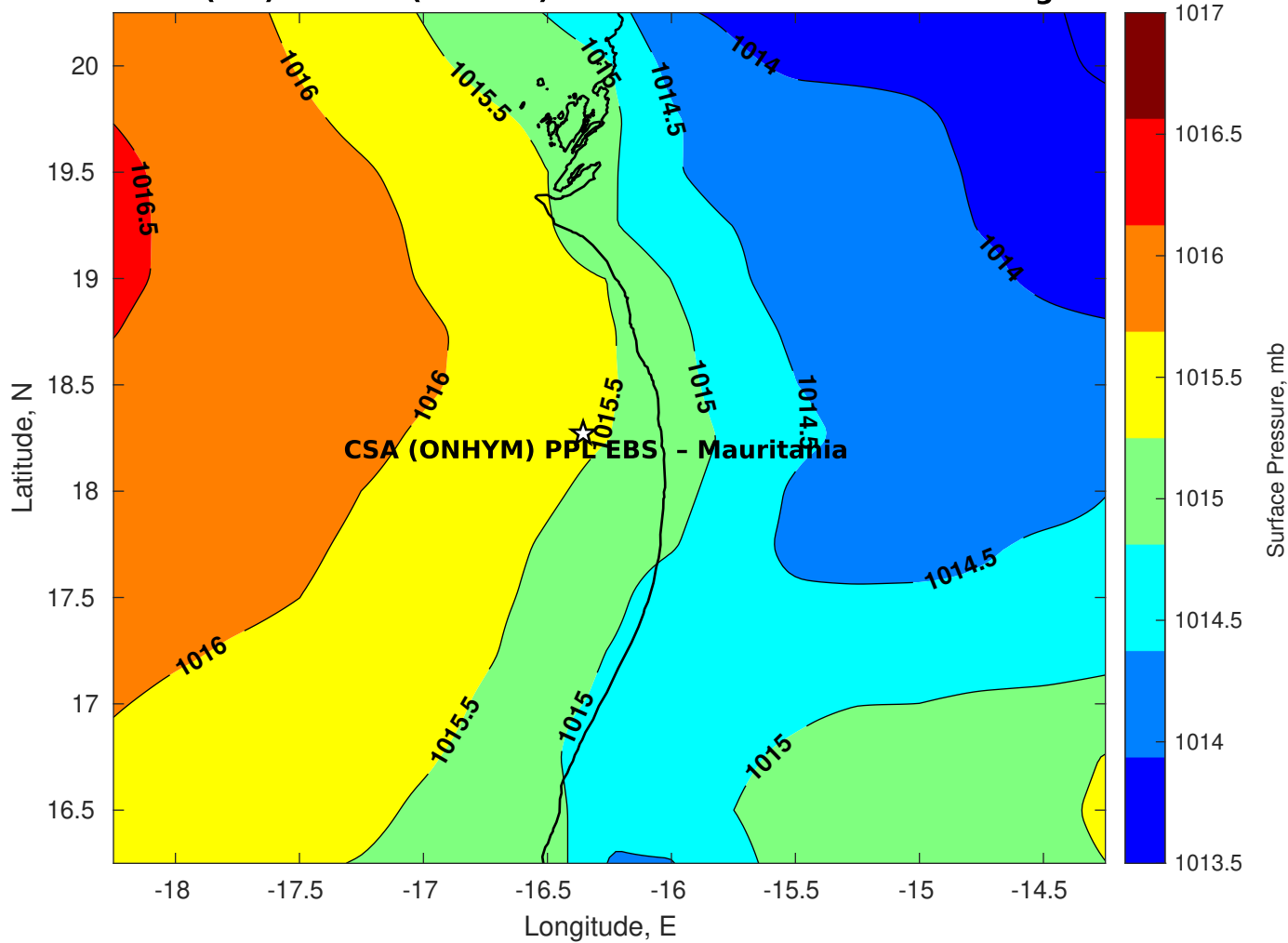
Surface Pressure (mb) for CSA (ONHYM) PPL EBS - Mauritania at 03-Aug-2025 12:00:00
