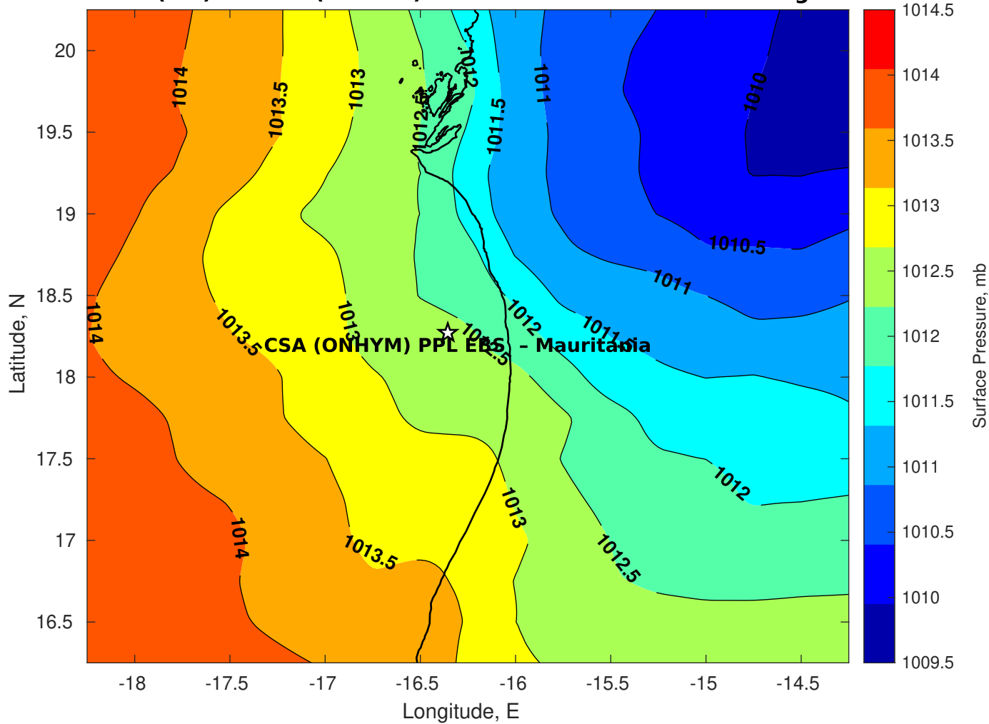
Surface Pressure (mb) for CSA (ONHYM) PPL EBS - Mauritania at 01-Aug-2025 12:00:00
