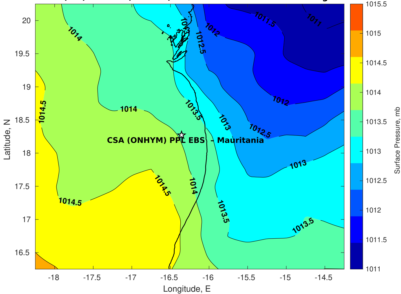
Surface Pressure (mb) for CSA (ONHYM) PPL EBS - Mauritania at 02-Aug-2025 12:00:00
