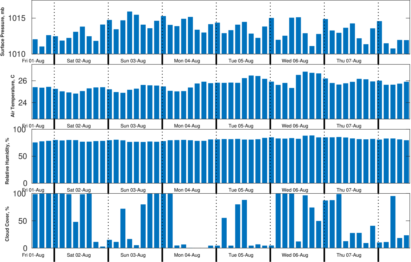
Met Forecast for CSA (ONHYM) PPL EBS - Mauritania from 01-Aug-2025 12:00:00 to 08-Aug-2025 12:00:00
