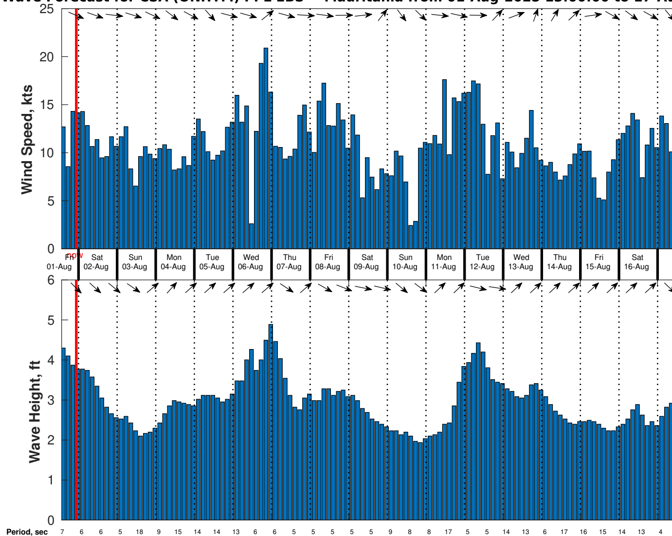
Wind & Wave Forecast for CSA (ONHYM) PPL EBS - Mauritania from 01-Aug-2025 13:00:00 to 17-Aug-2025 13:00:00
