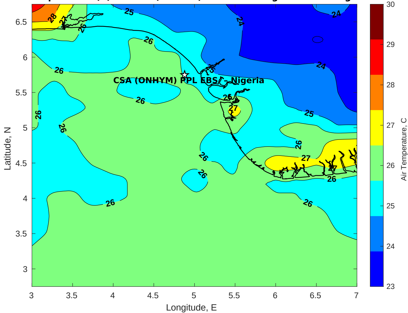
Air Temperature (C) for CSA (ONHYM) PPL EBS - Nigeria at 01-Aug-2025
