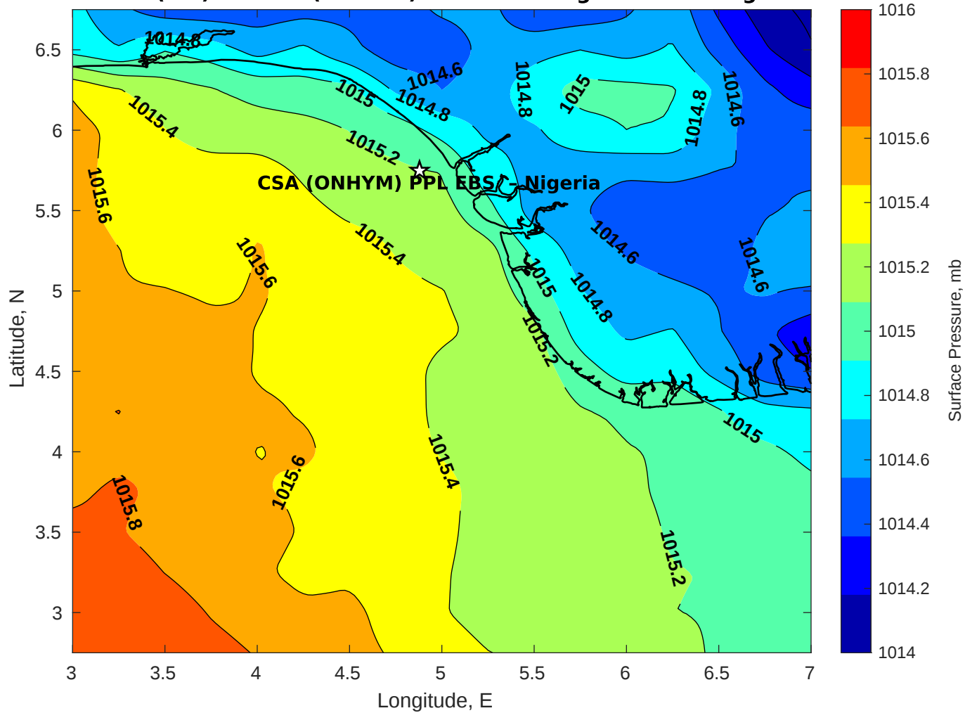
Surface Pressure (mb) for CSA (ONHYM) PPL EBS - Nigeria at 02-Aug-2025 12:00:00
