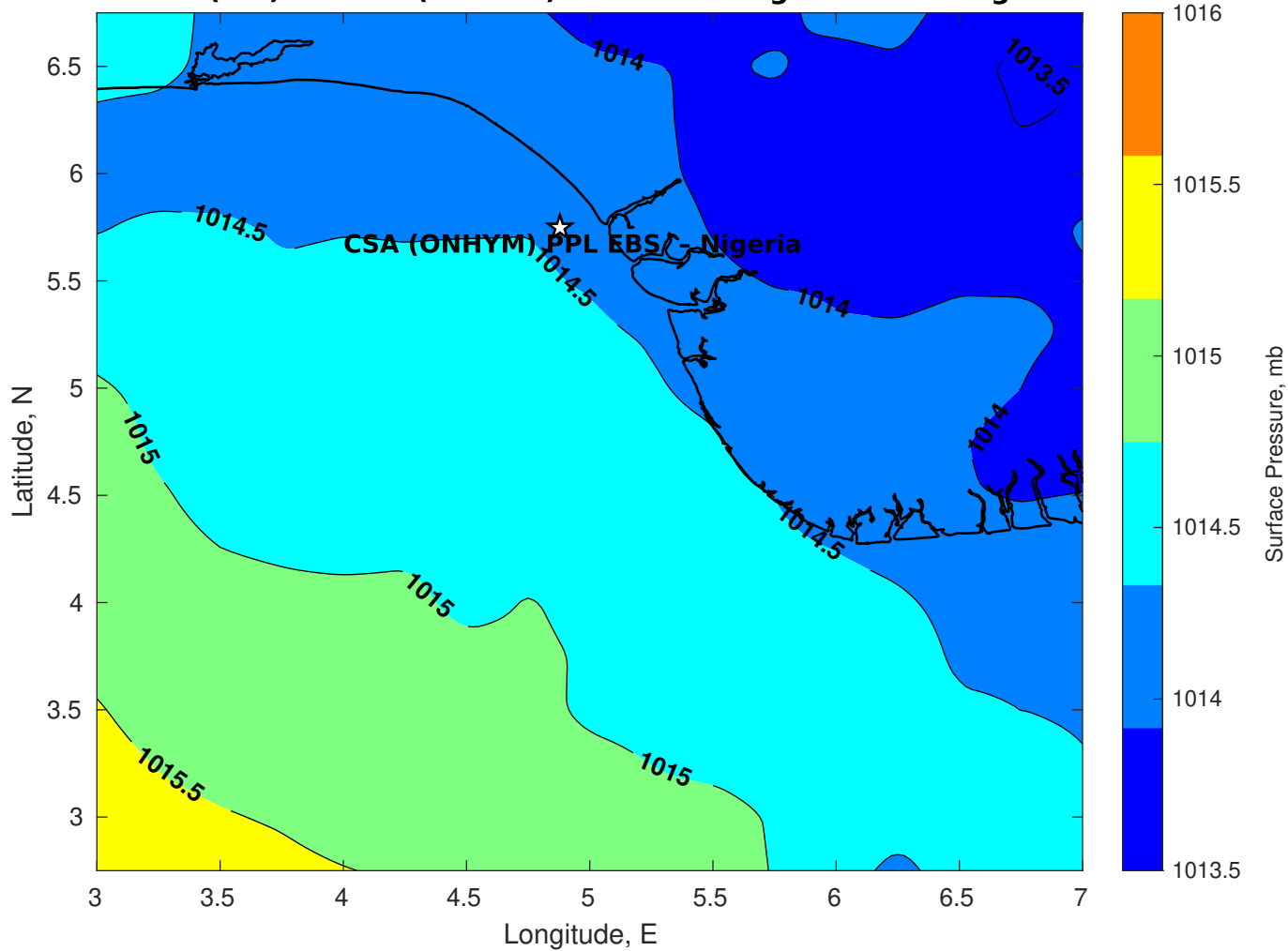
Surface Pressure (mb) for CSA (ONHYM) PPL EBS - Nigeria at 03-Aug-2025 12:00:00
