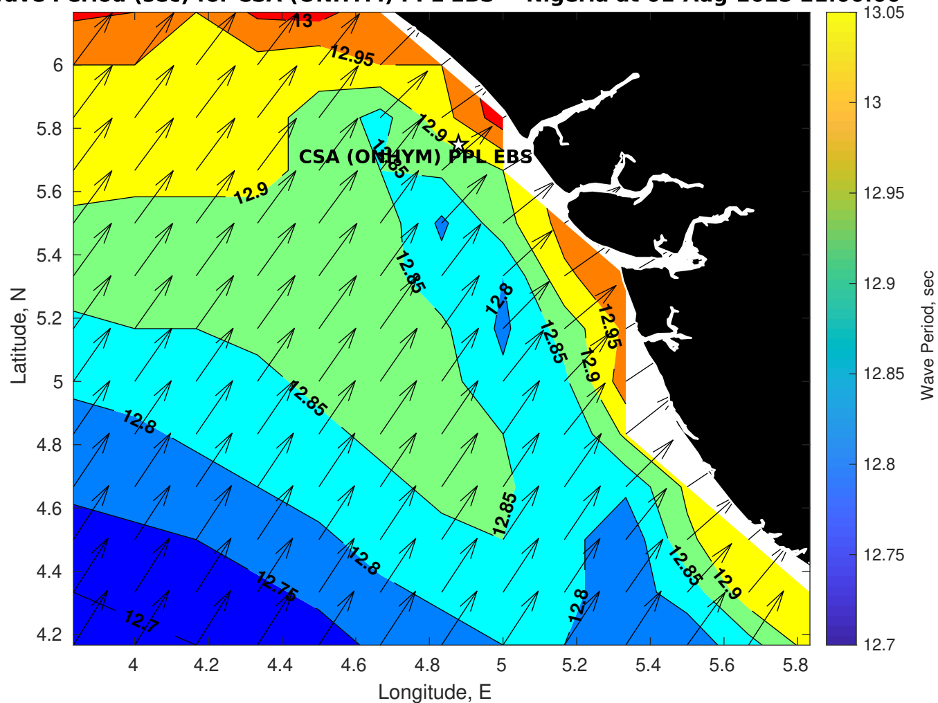
Wave Period (sec) for CSA (ONHYM) PPL EBS - Nigeria at 01-Aug-2025 21:00:00
