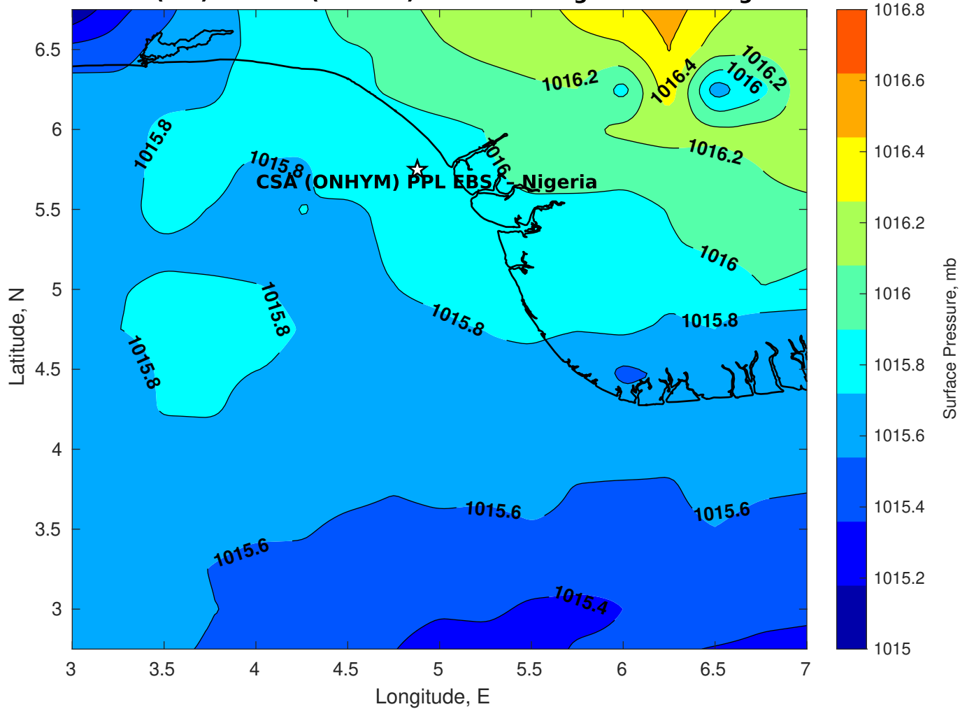
Surface Pressure (mb) for CSA (ONHYM) PPL EBS - Nigeria at 01-Aug-2025 12:00:00
