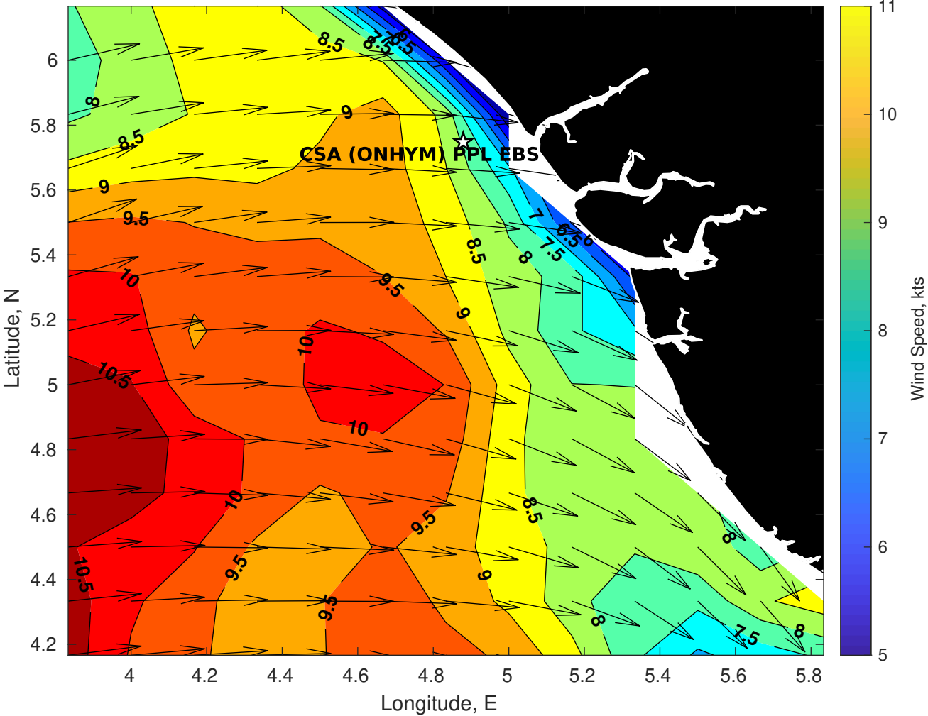
Winds (kts) for CSA (ONHYM) PPL EBS - Nigeria at 01-Aug-2025 21:00:00
