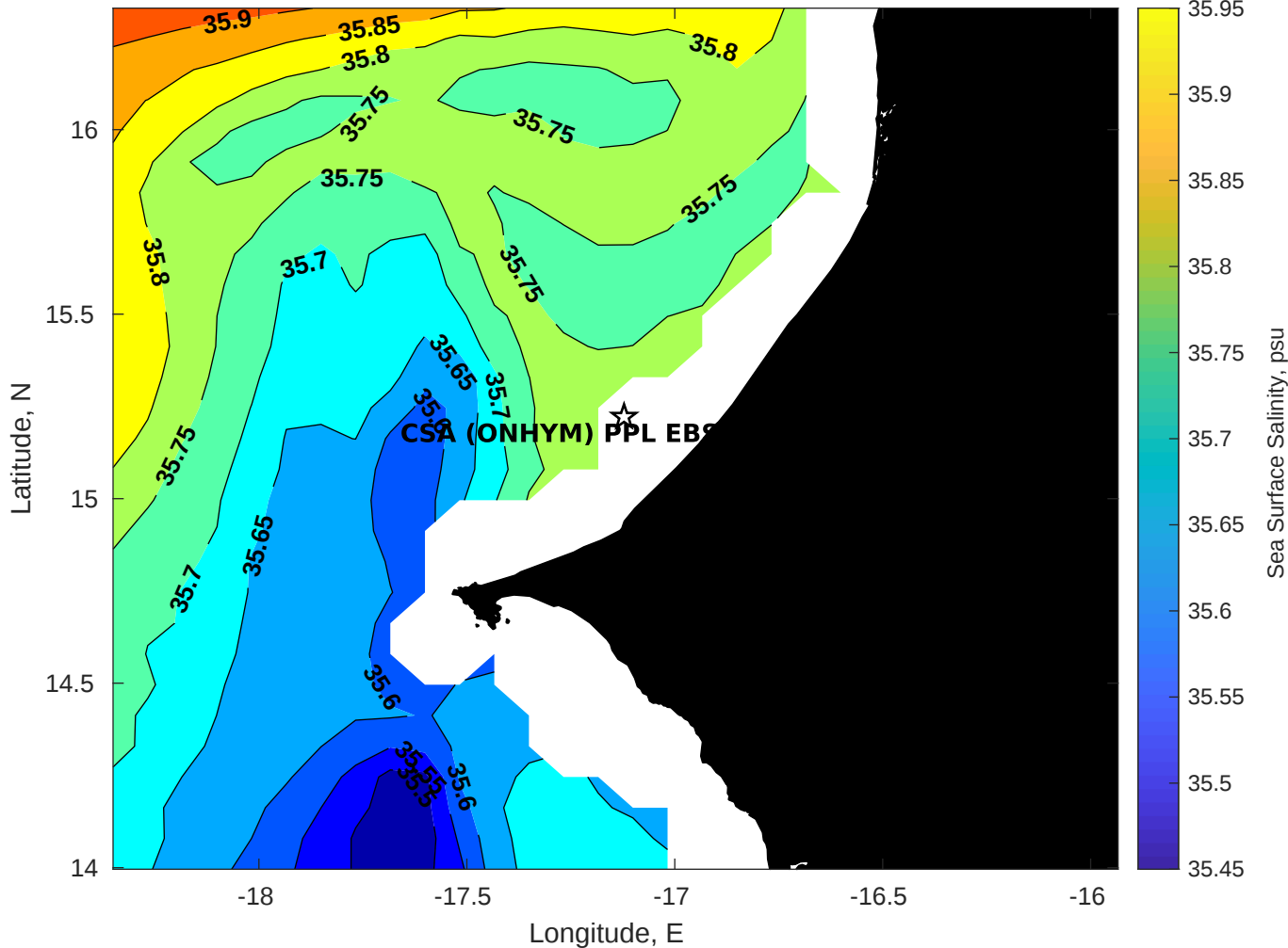
Surface Salinity for CSA (ONHYM) PPL EBS - Senegal at 01-Aug-2025 00:00:00
