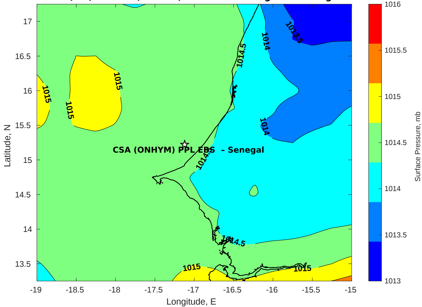
Surface Pressure (mb) for CSA (ONHYM) PPL EBS - Senegal at 02-Aug-2025 12:00:00
