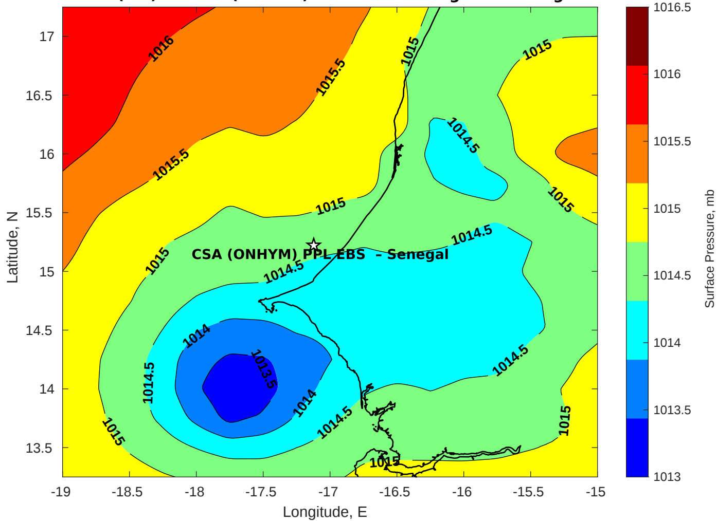
Surface Pressure (mb) for CSA (ONHYM) PPL EBS - Senegal at 03-Aug-2025 12:00:00
