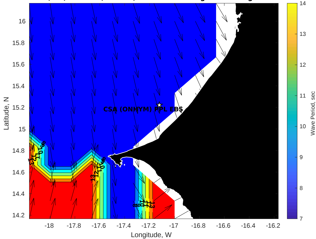
Wave Period (sec) for CSA (ONHYM) PPL EBS - Senegal at 01-Aug-2025 21:00:00
