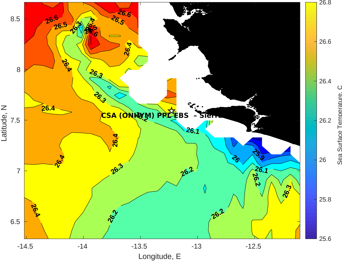
SST for CSA (ONHYM) PPL EBS - Sierra Leone at 01-Aug-2025 00:00:00
