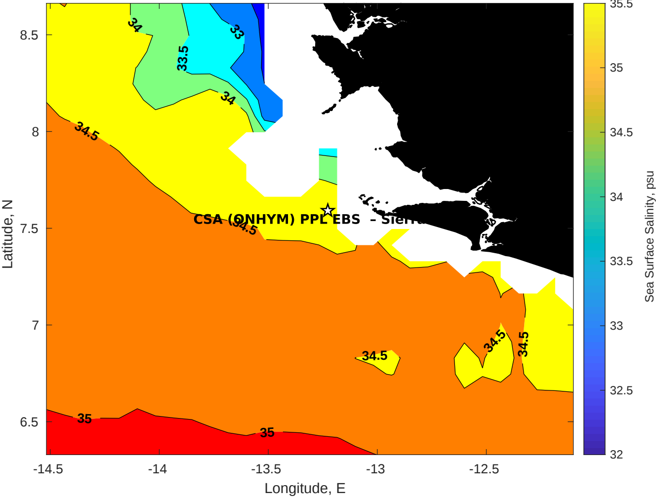
Surface Salinity for CSA (ONHYM) PPL EBS - Sierra Leone at 01-Aug-2025 00:00:00
