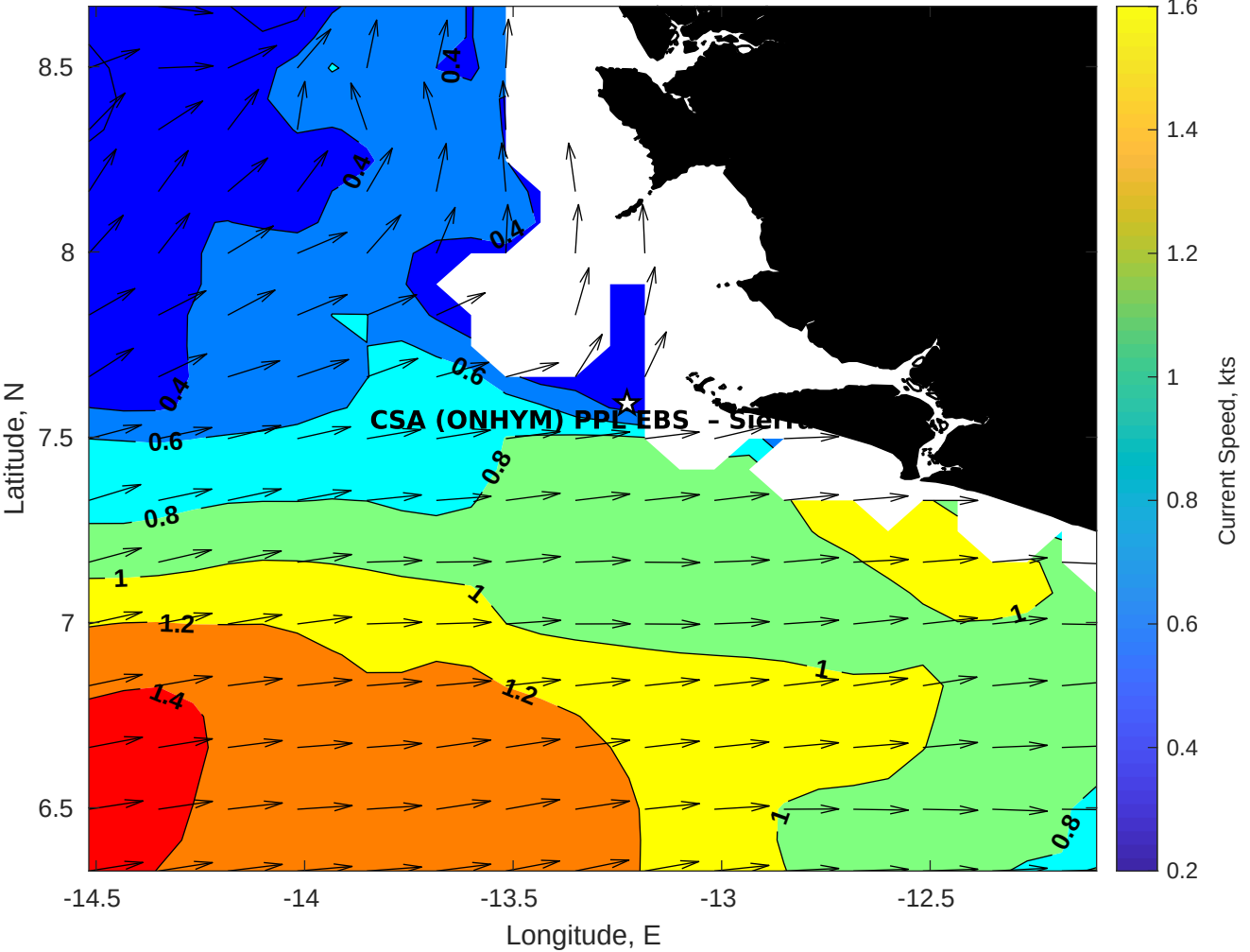
Surface Currents for CSA (ONHYM) PPL EBS - Sierra Leone at 01-Aug-2025 00:00:00
