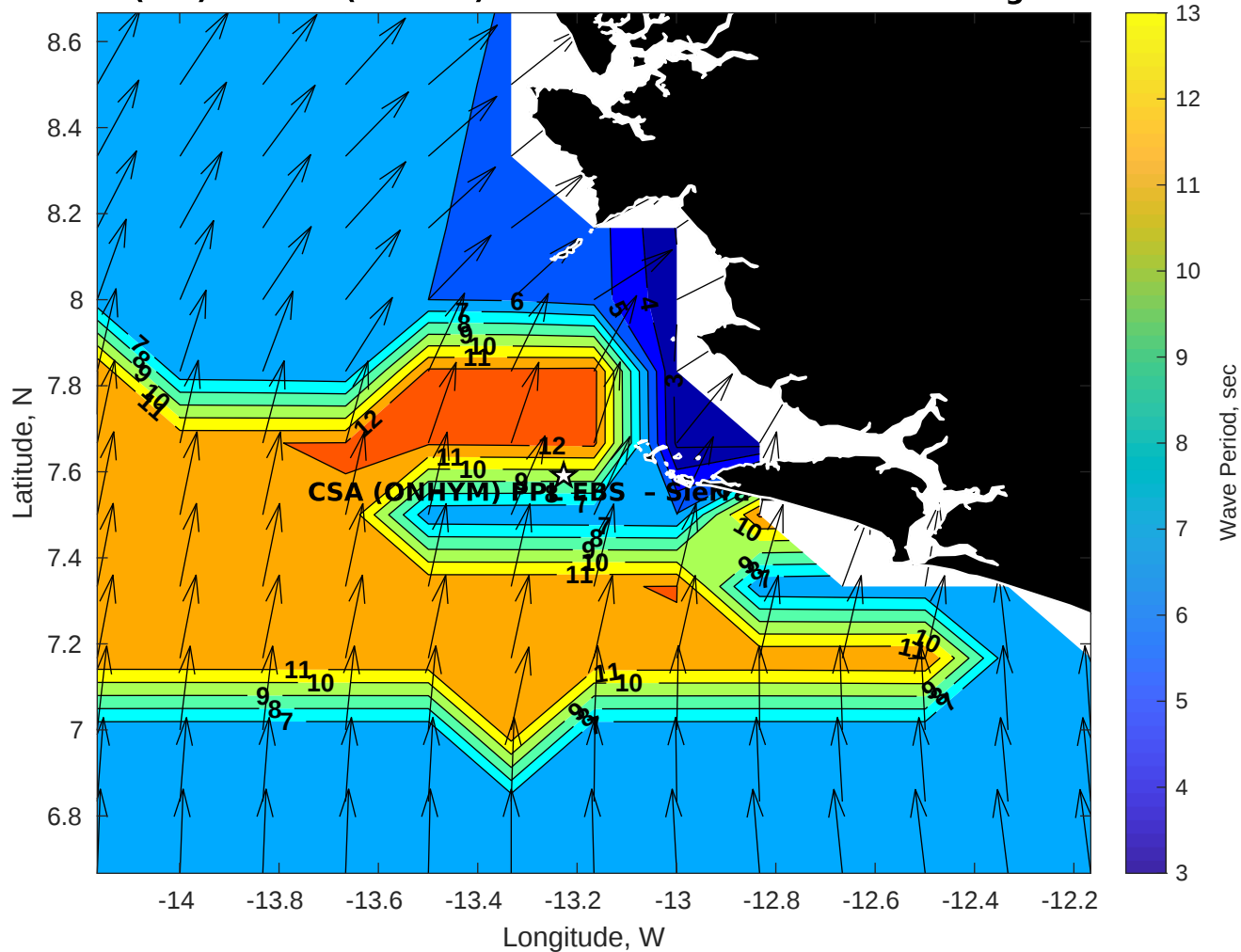
Wave Period (sec) for CSA (ONHYM) PPL EBS - Sierra Leone at 01-Aug-2025 21:00:00
