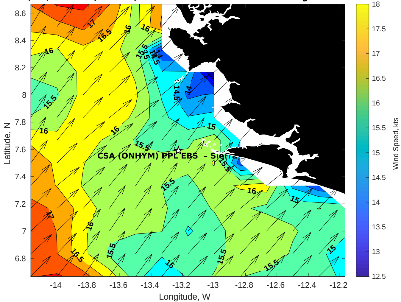
Winds (kts) for CSA (ONHYM) PPL EBS - Sierra Leone at 01-Aug-2025 21:00:00
