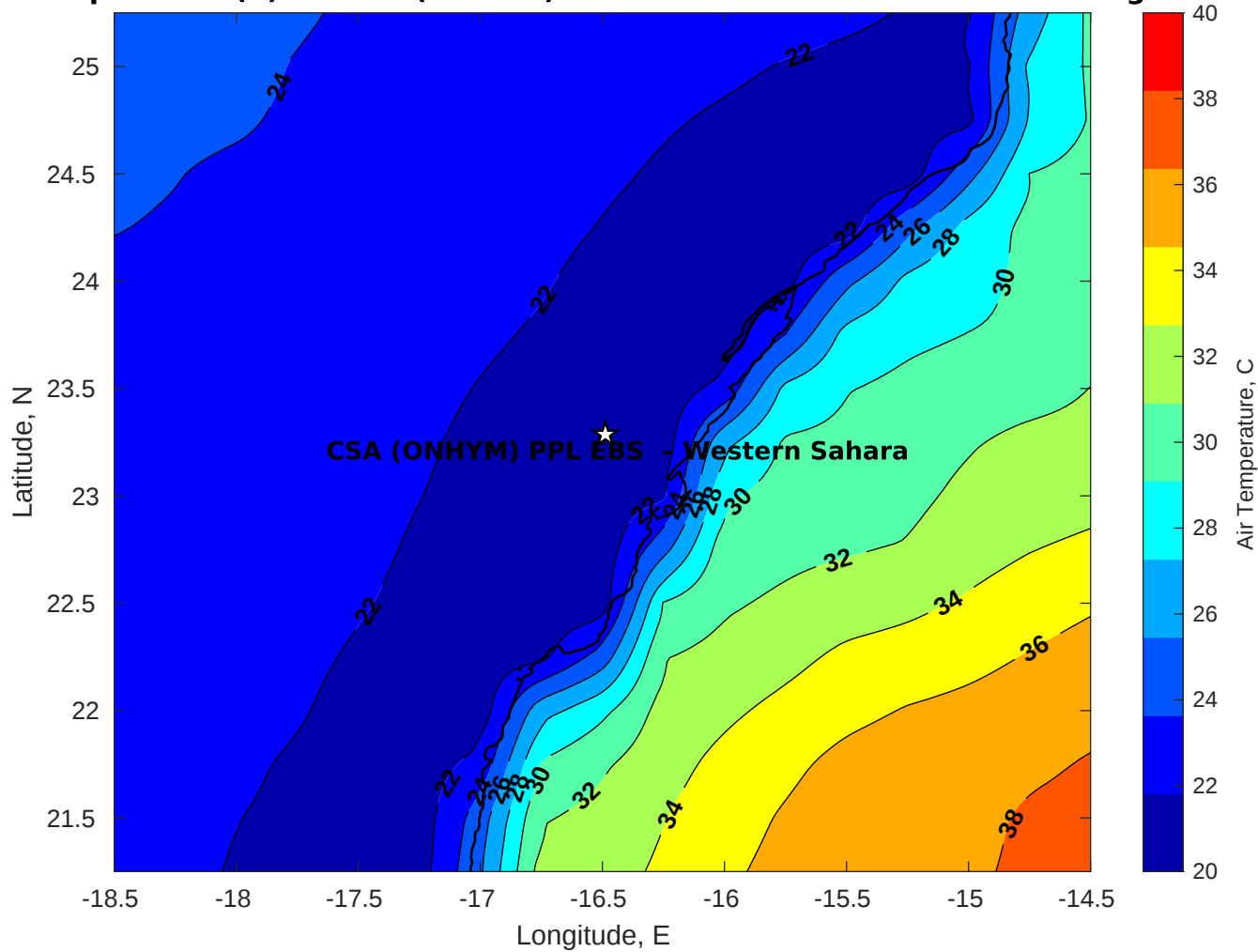
Air Temperature (C) for CSA (ONHYM) PPL EBS - Western Sahara at 01-Aug-2025
