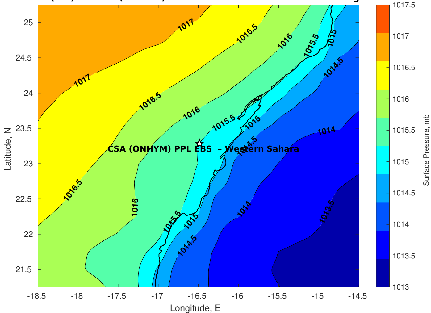
Surface Pressure (mb) for CSA (ONHYM) PPL EBS - Western Sahara at 03-Aug-2025 12:00:00
