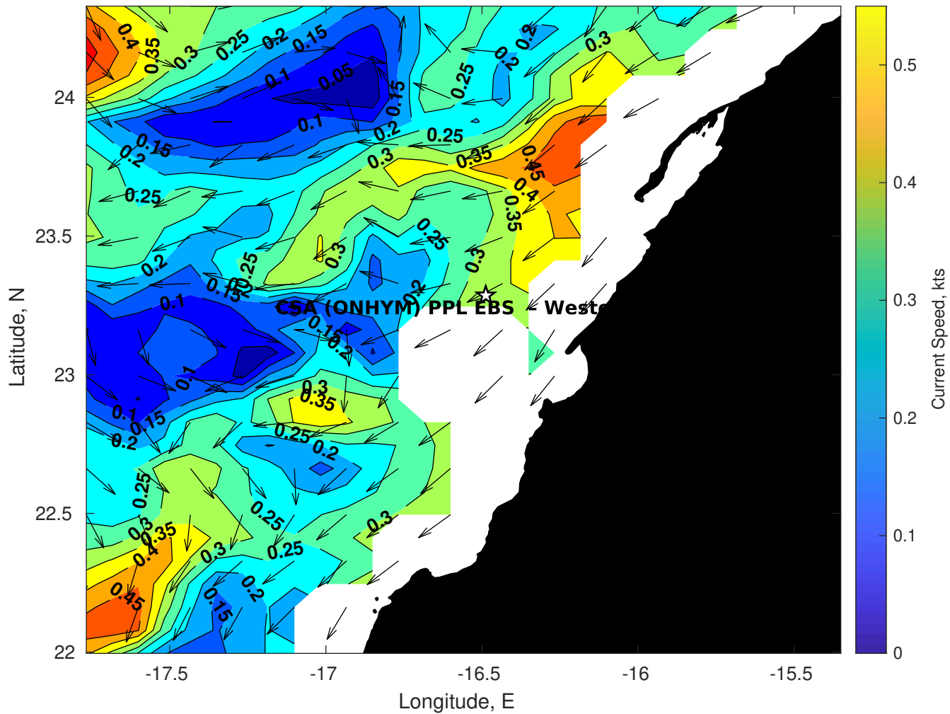
Surface Currents for CSA (ONHYM) PPL EBS - Western Sahara at 01-Aug-2025 00:00:00
