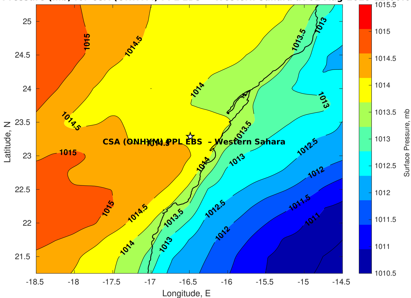
Surface Pressure (mb) for CSA (ONHYM) PPL EBS - Western Sahara at 01-Aug-2025 12:00:00
