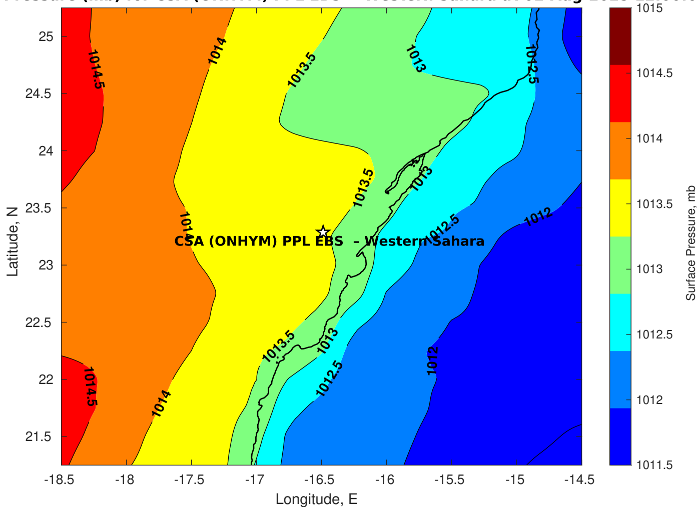
Surface Pressure (mb) for CSA (ONHYM) PPL EBS - Western Sahara at 02-Aug-2025 12:00:00
