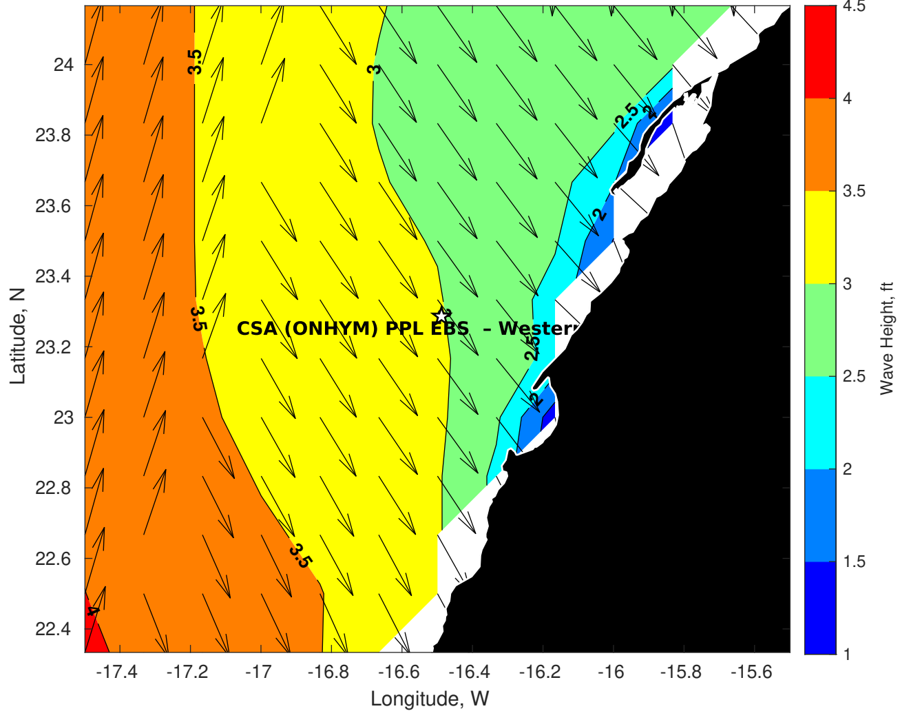
Wave Height (ft) for CSA (ONHYM) PPL EBS - Western Sahara at 01-Aug-2025 21:00:00
