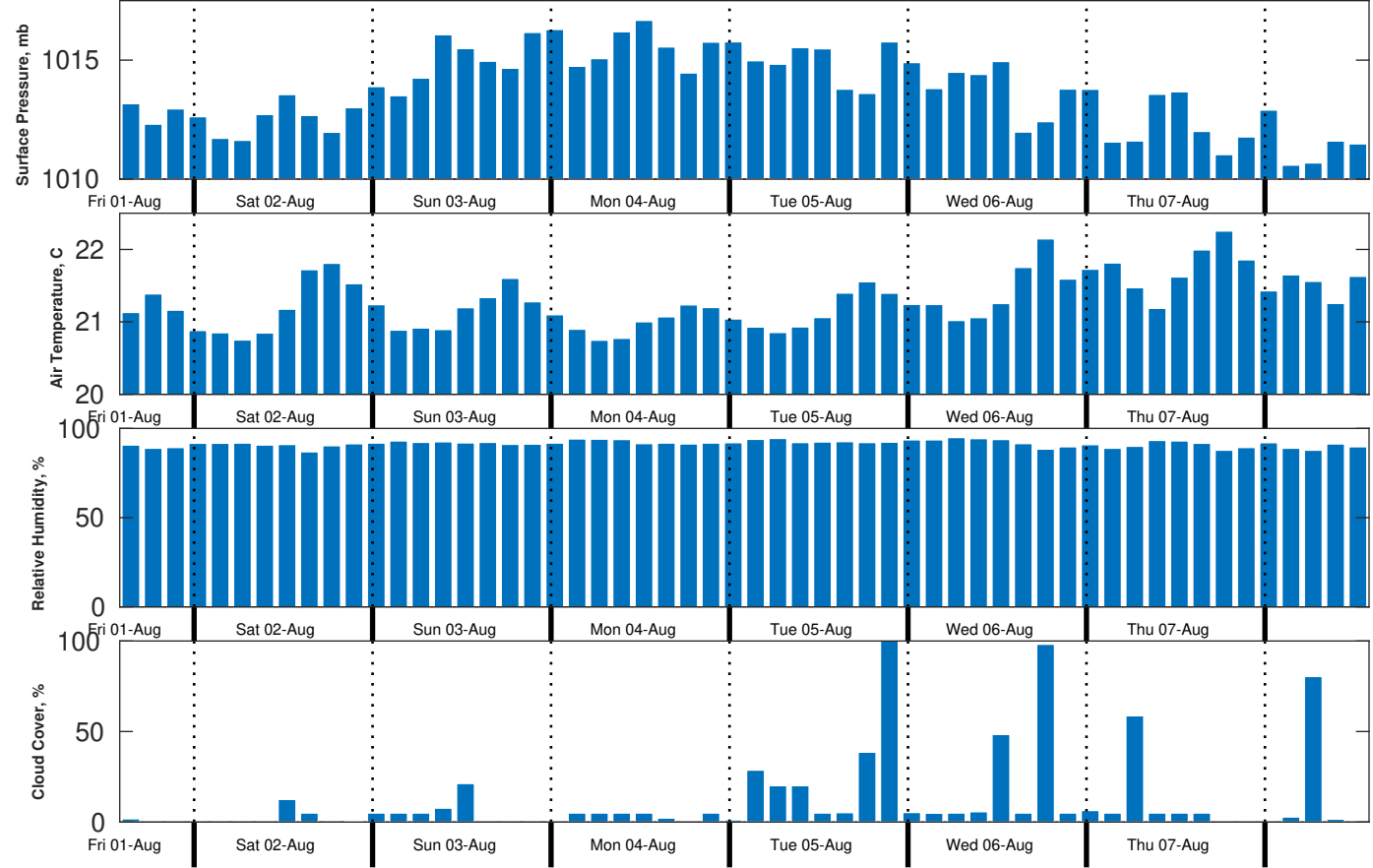
Met Forecast for CSA (ONHYM) PPL EBS - Western Sahara from 01-Aug-2025 12:00:00 to 08-Aug-2025 12:00:00
