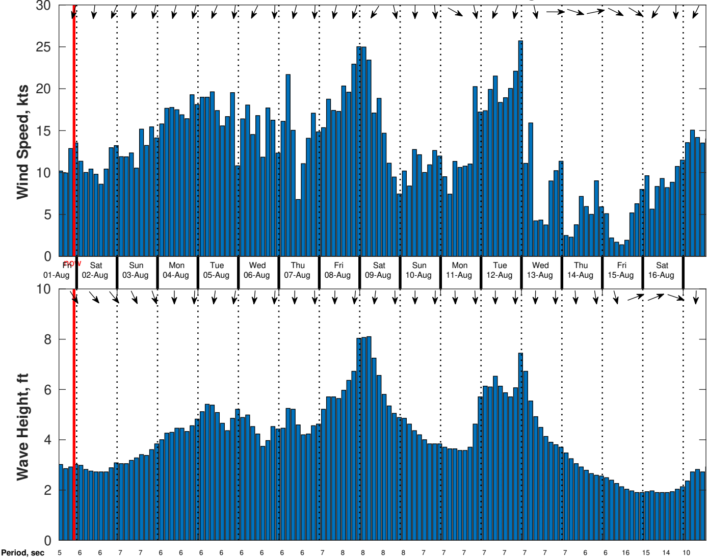
Wind & Wave Forecast for CSA (ONHYM) PPL EBS - Western Sahara from 01-Aug-2025 13:00:00 to 17-Aug-2025 13:00:00
