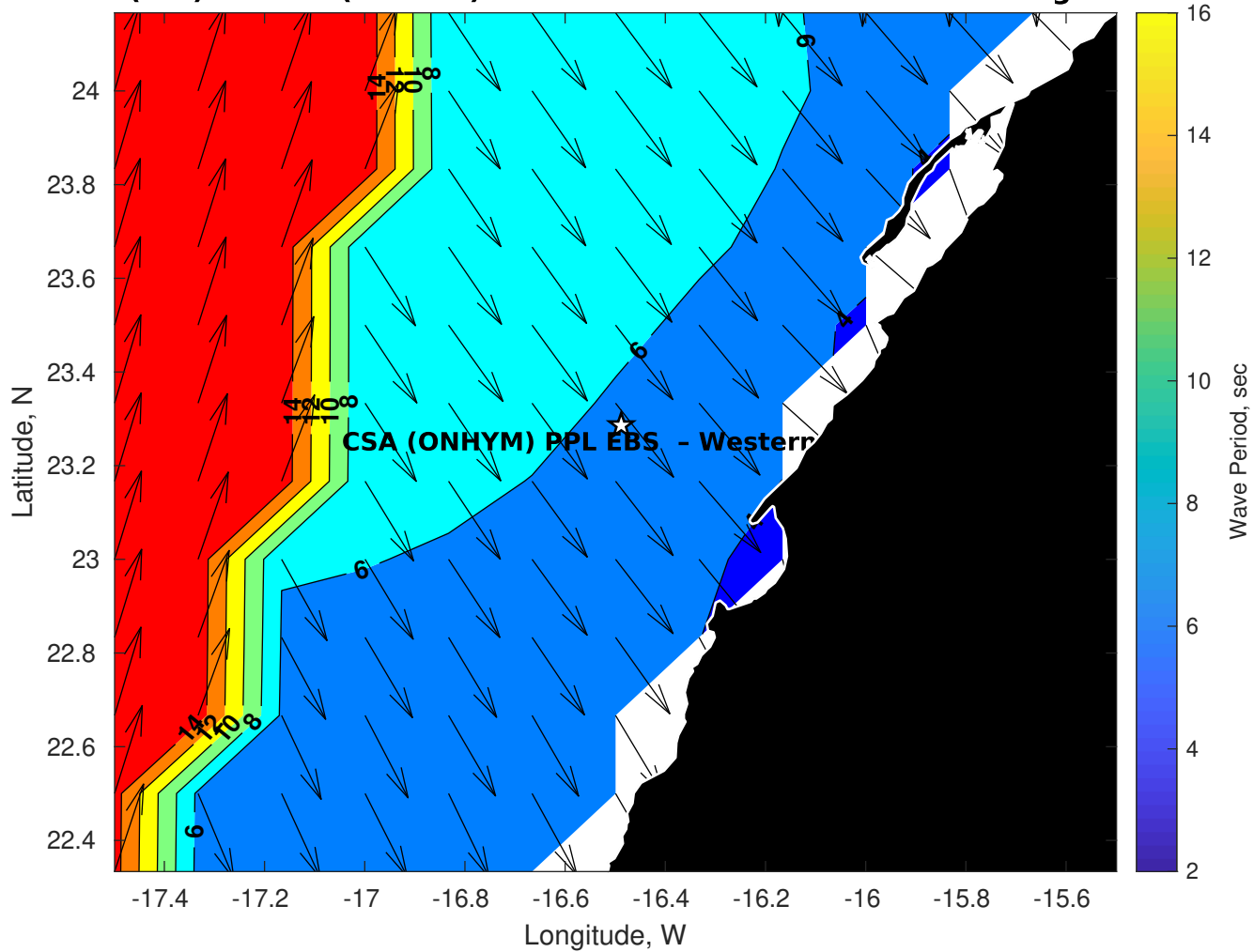
Wave Period (sec) for CSA (ONHYM) PPL EBS - Western Sahara at 01-Aug-2025 21:00:00
