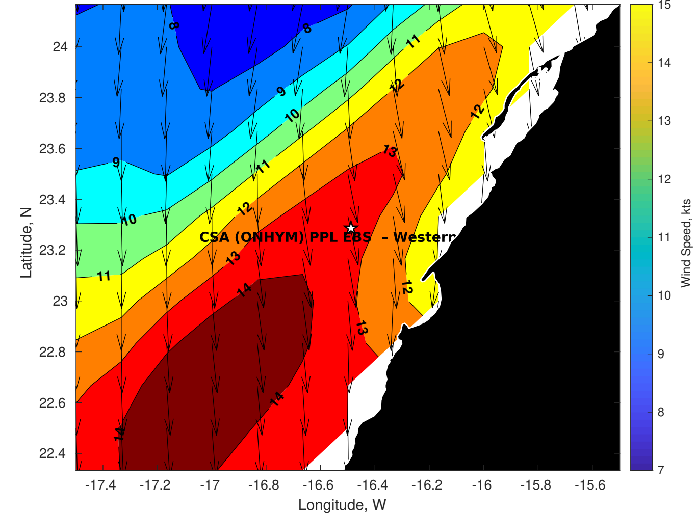
Winds (kts) for CSA (ONHYM) PPL EBS - Western Sahara at 01-Aug-2025 21:00:00
