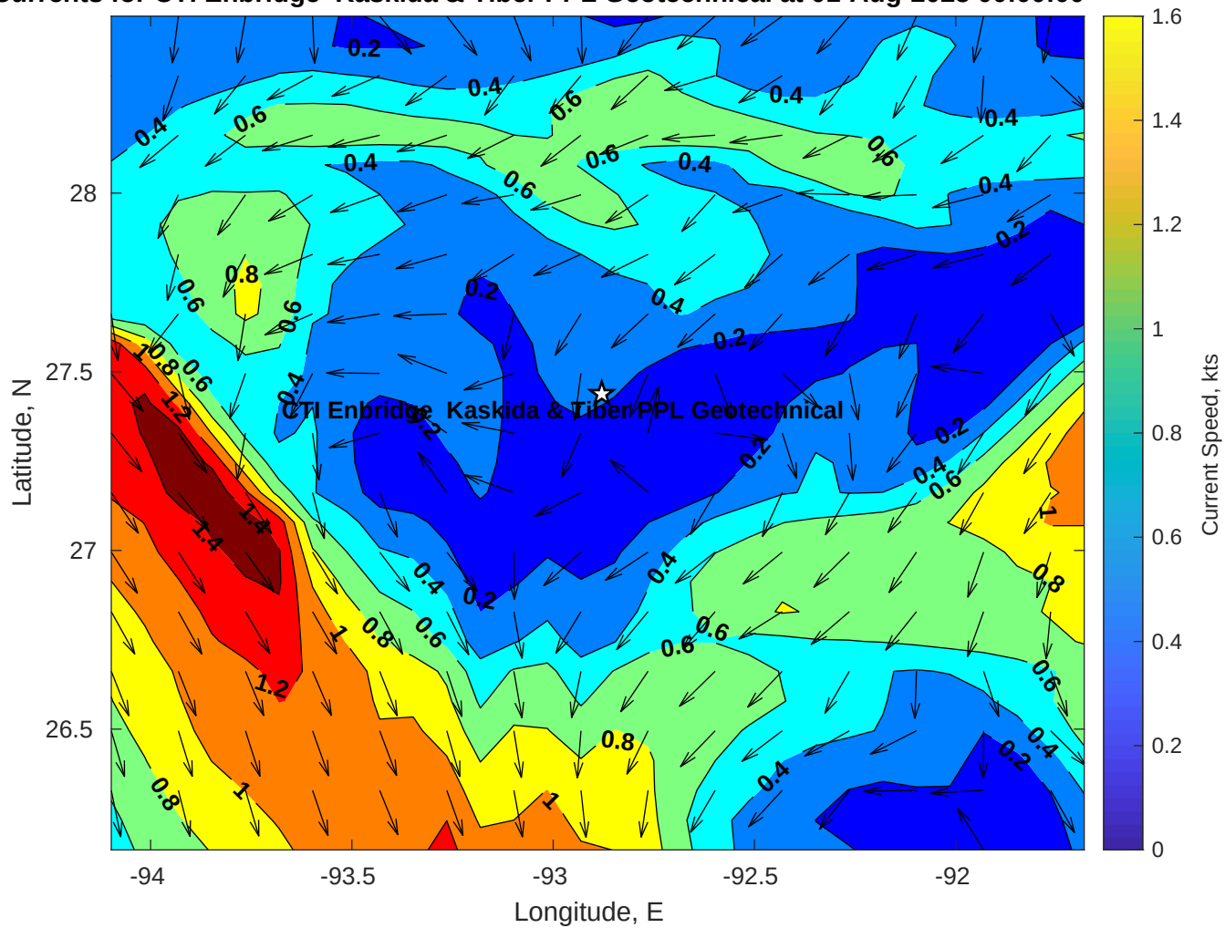
Surface Currents for CTI Enbridge Kaskida & Tiber PPL Geotechnical at 01-Aug-2025 00:00:00
