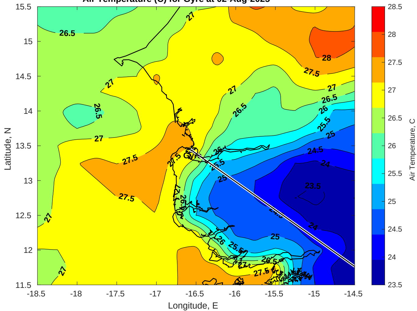
Air Temperature (C) for Gyre at 02-Aug-2025
