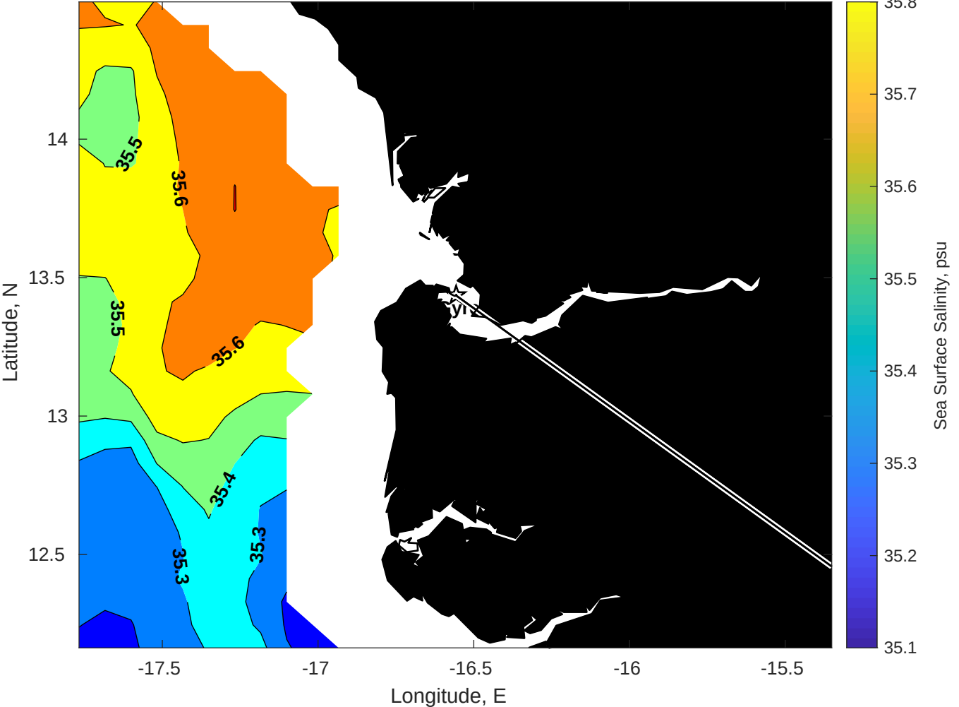
Surface Salinity for Gyre at 01-Aug-2025 00:00:00
