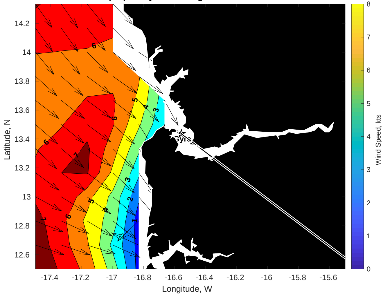
Winds (kts) for Gyre at 02-Aug-2025 09:00:00
