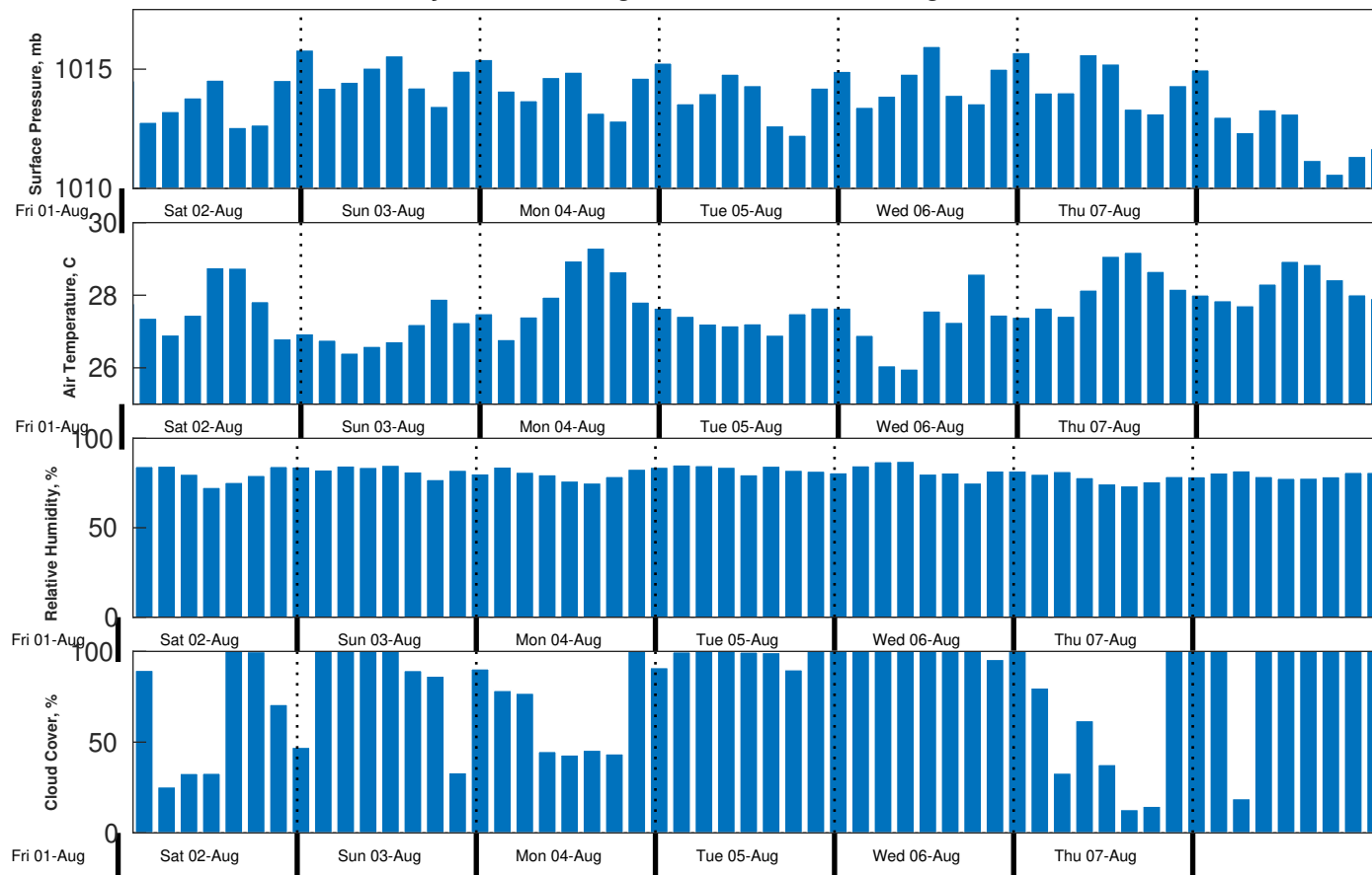
Met Forecast for Gyre from 01-Aug-2025 23:00:00 to 08-Aug-2025 23:00:00
