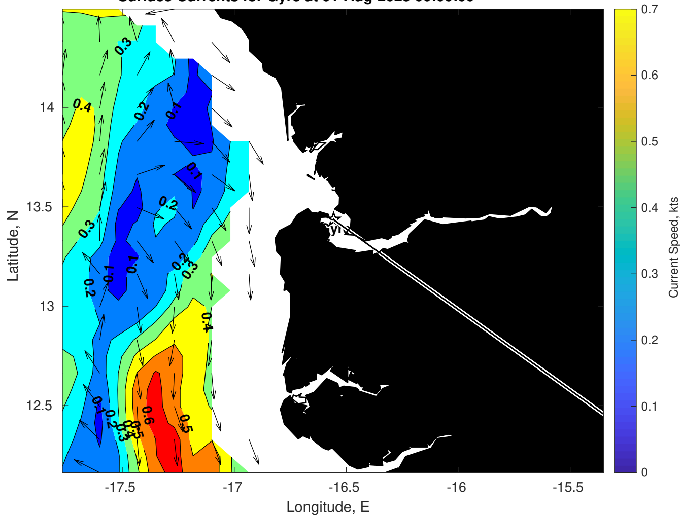
Surface Currents for Gyre at 01-Aug-2025 00:00:00
