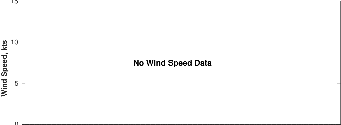
Wind & Wave Forecast for Gyre from 01-Aug-2025 23:00:00 to 17-Aug-2025 23:00:00
