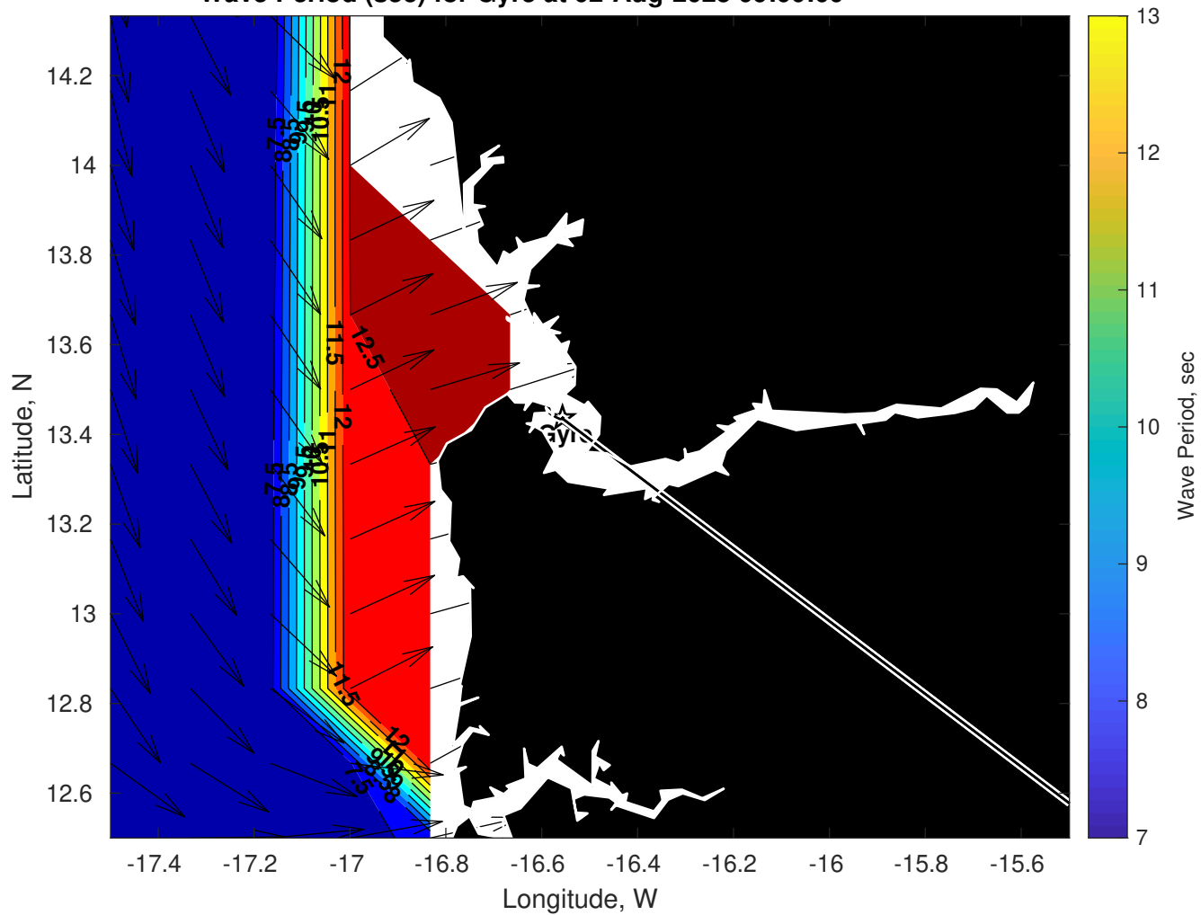
Wave Period (sec) for Gyre at 02-Aug-2025 09:00:00
