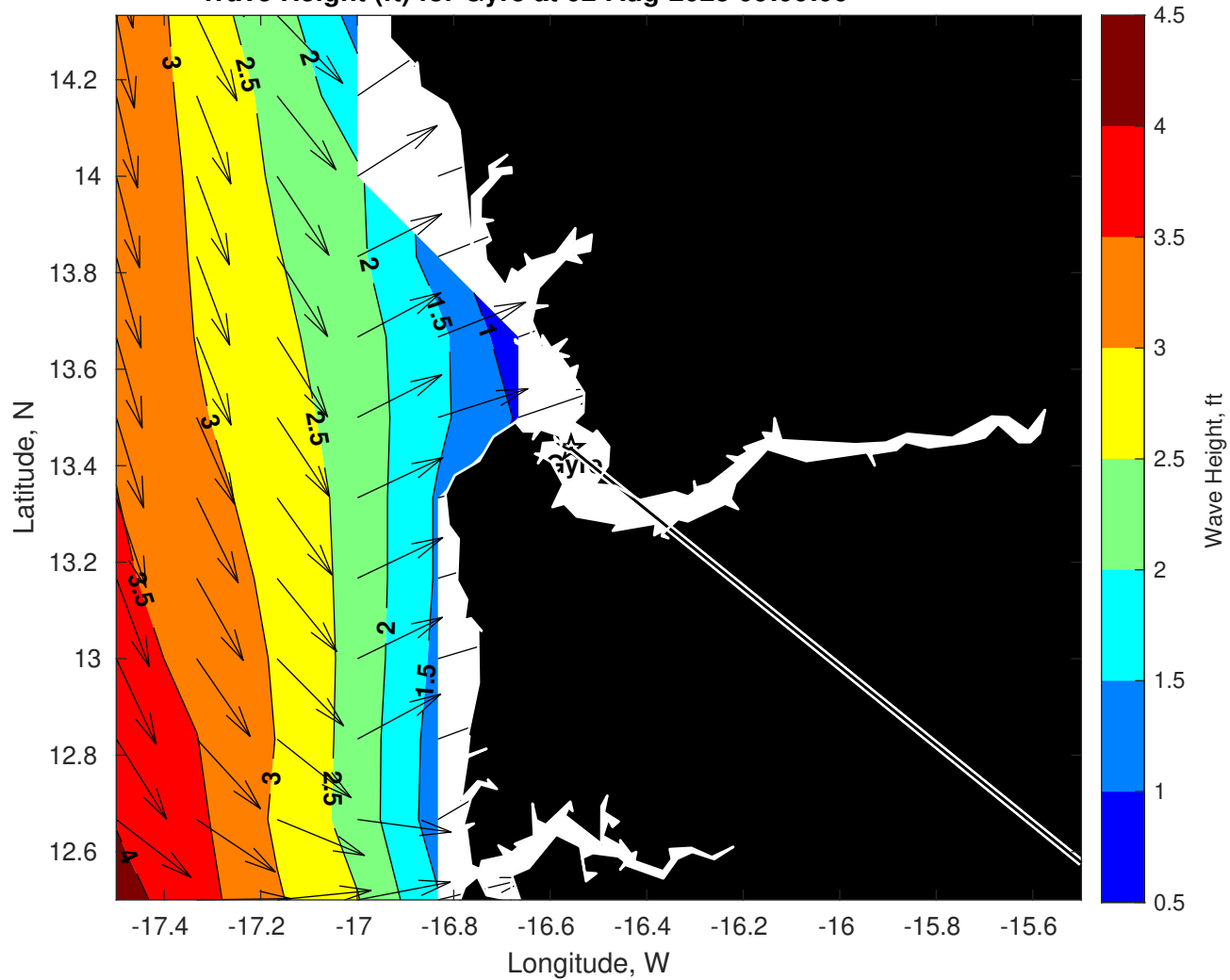
Wave Height (ft) for Gyre at 02-Aug-2025 09:00:00
