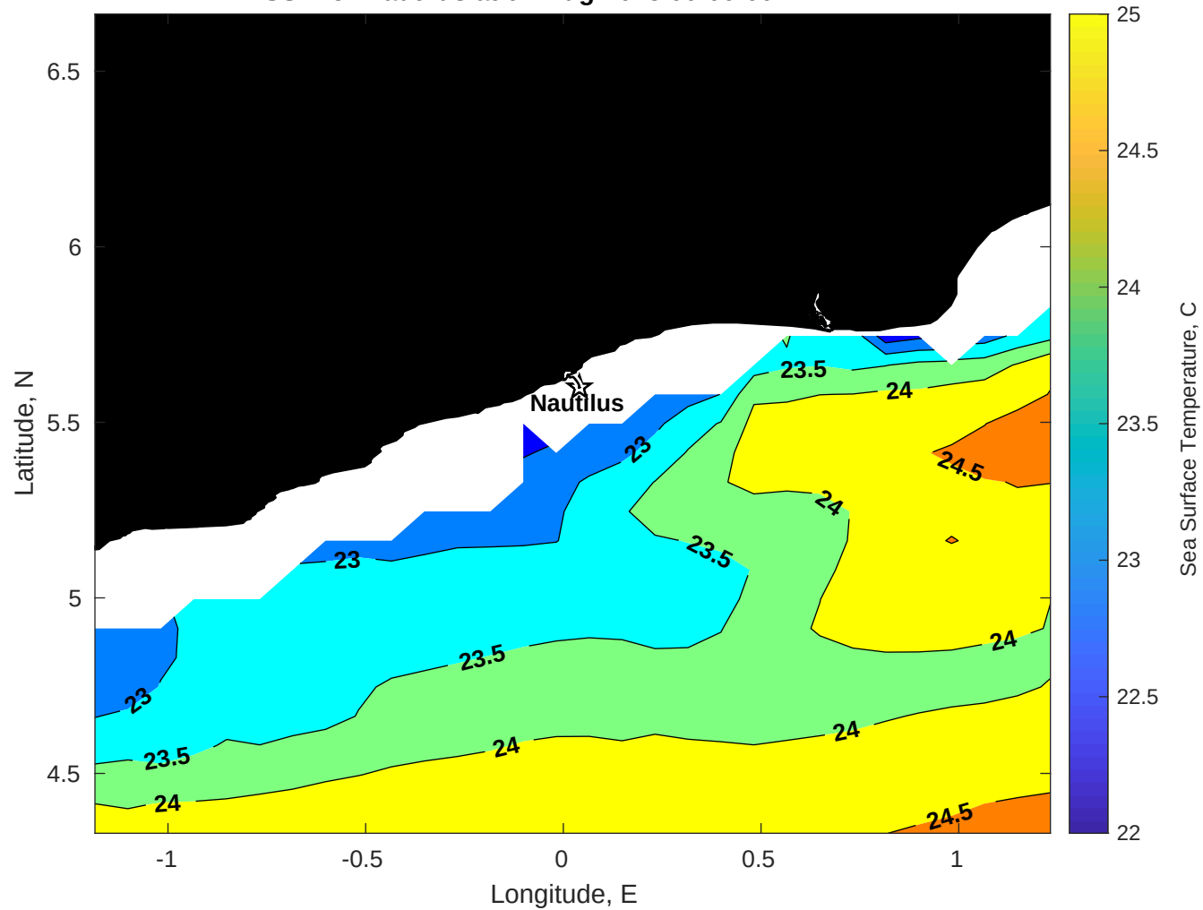
SST for Nautilus at 01-Aug-2025 00:00:00
