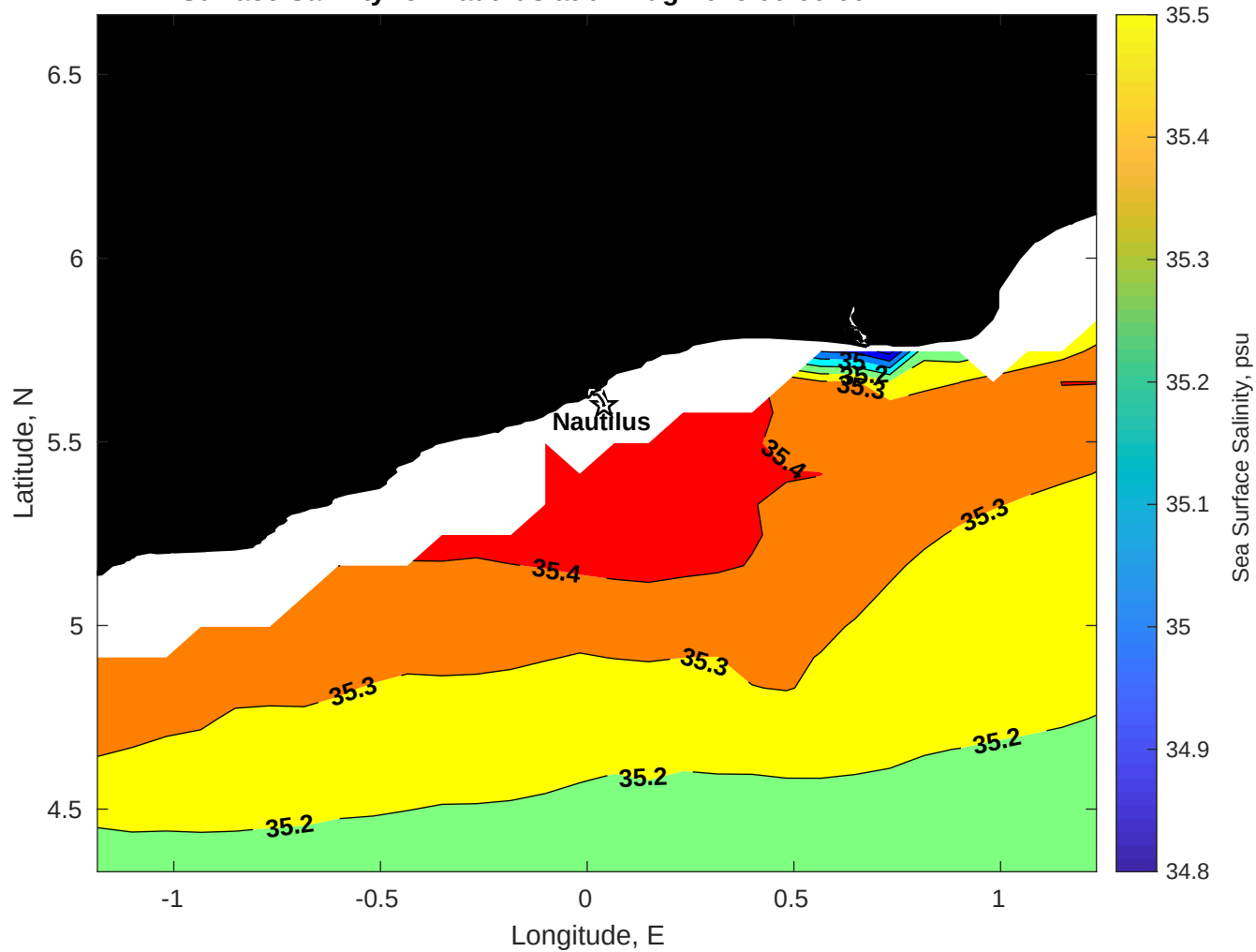
Surface Salinity for Nautilus at 01-Aug-2025 00:00:00
