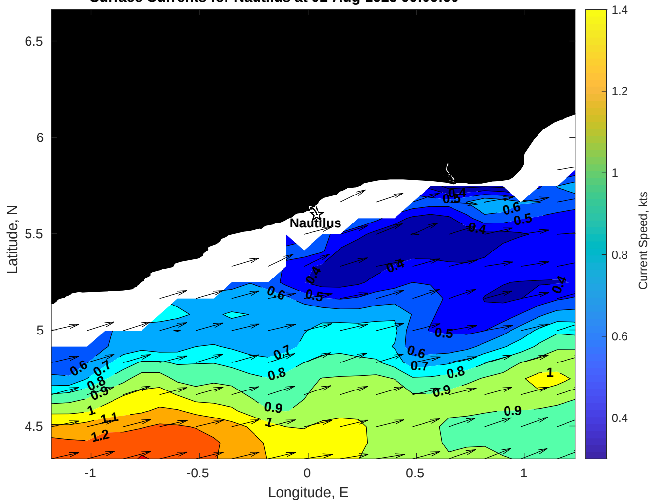
Surface Currents for Nautilus at 01-Aug-2025 00:00:00
