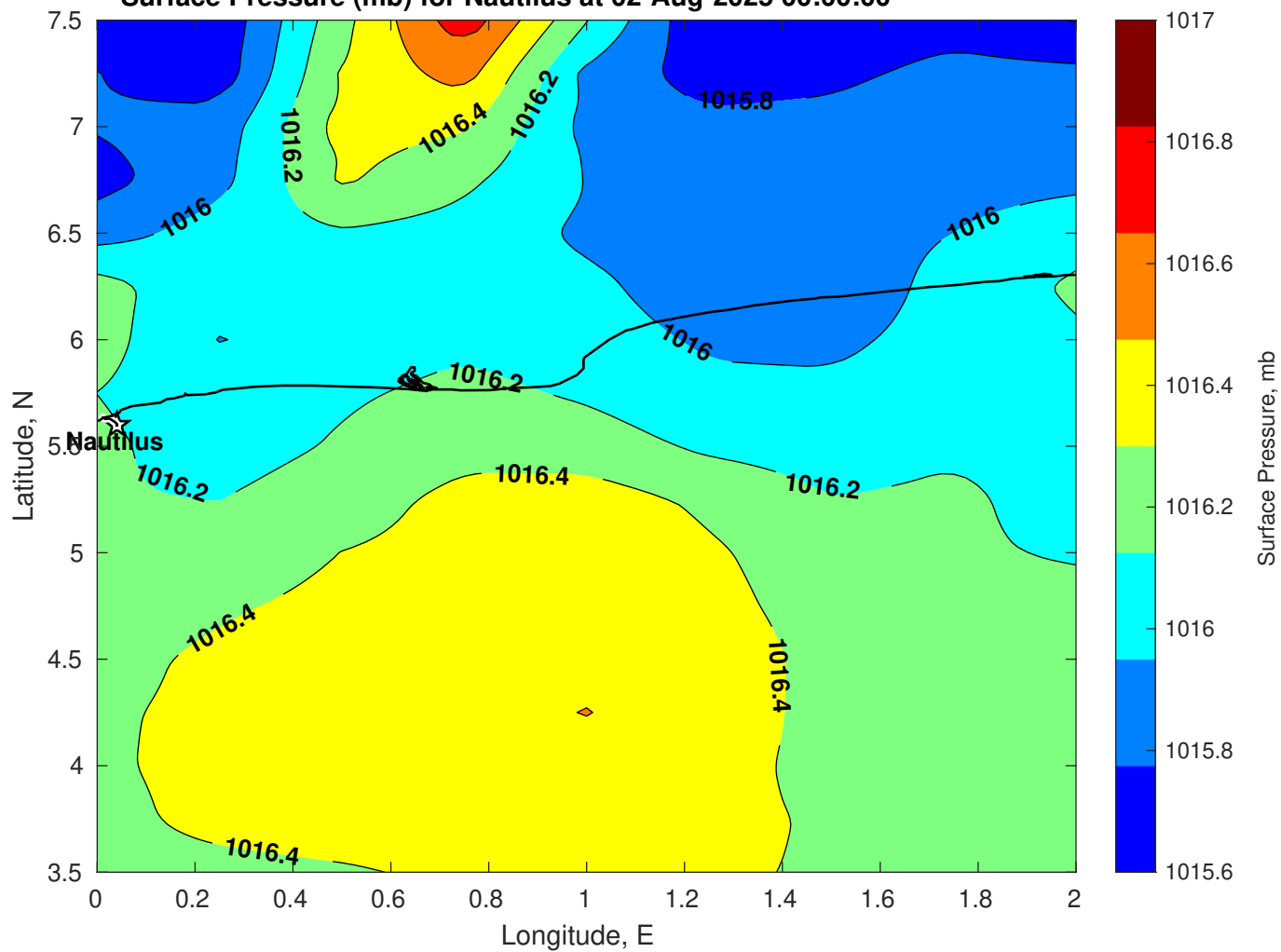
Surface Pressure (mb) for Nautilus at 02-Aug-2025 00:00:00
