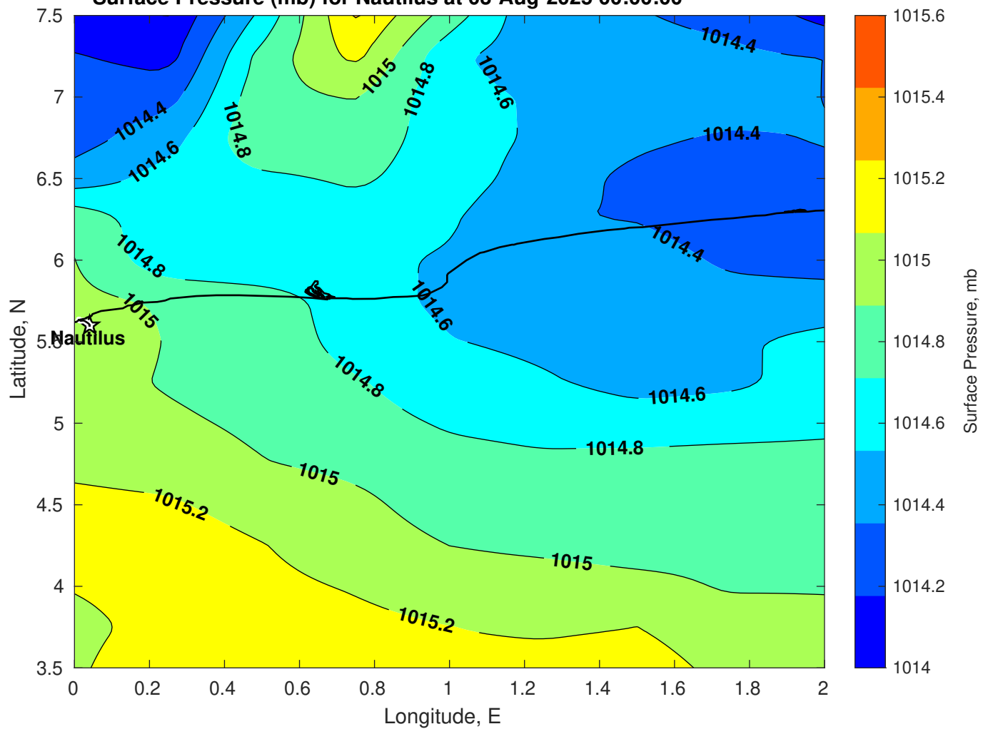
Surface Pressure (mb) for Nautilus at 03-Aug-2025 00:00:00
