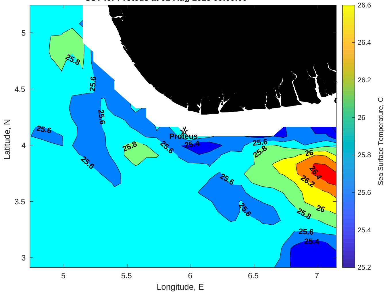
SST for Proteus at 01-Aug-2025 00:00:00
