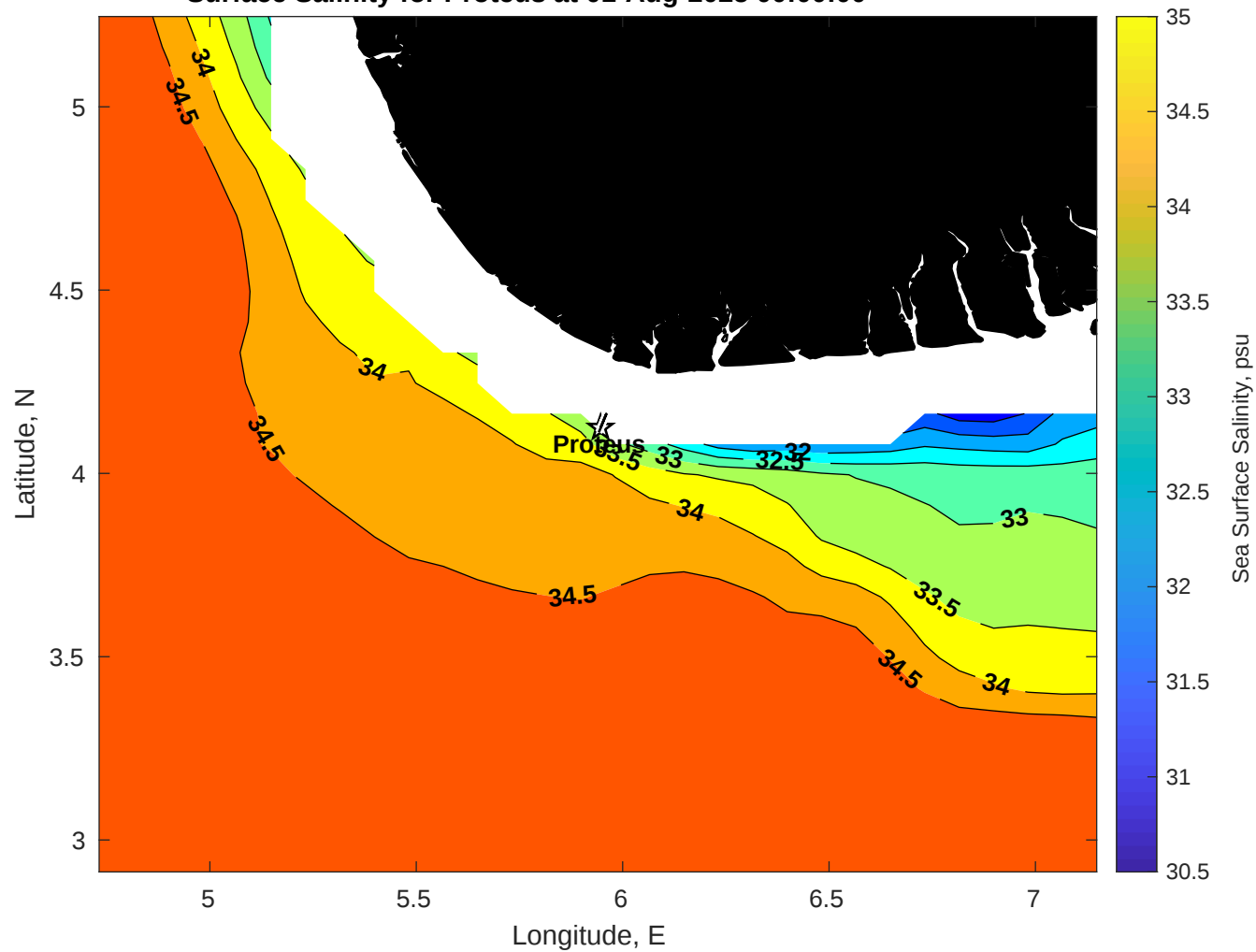
Surface Salinity for Proteus at 01-Aug-2025 00:00:00
